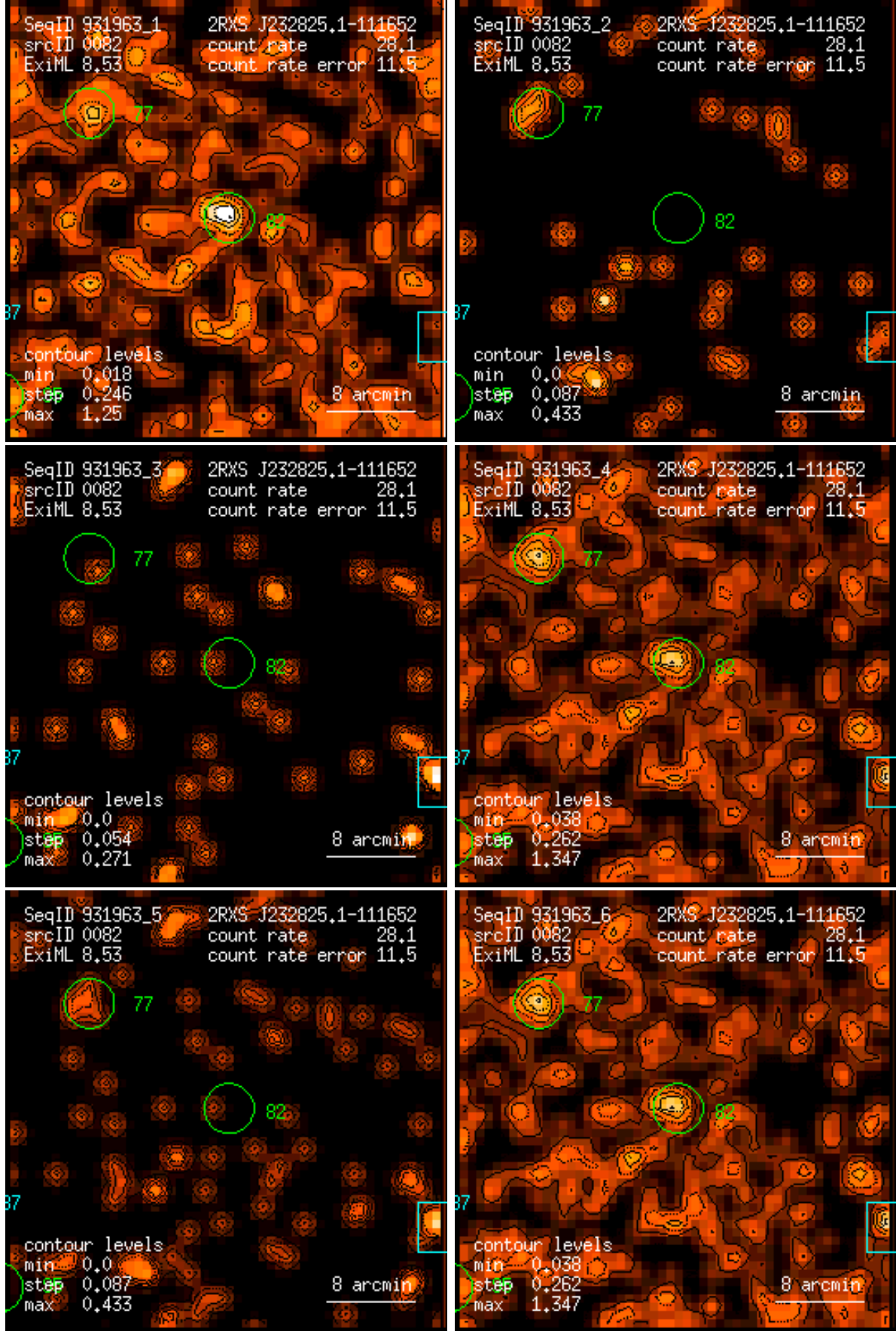
Figure 82: RASS 931963: detection 0082: band rate images, Gaussian filter: (1) PSPC channels 11 – 41, (2) 52 – 90, (3) 91 – 201, (4) 11 – 235, (5) 52 – 201, (6) 11 – 201. Broad band rates in counts/ks. Band rate contour levels in counts/ks/arcmin 2 .
