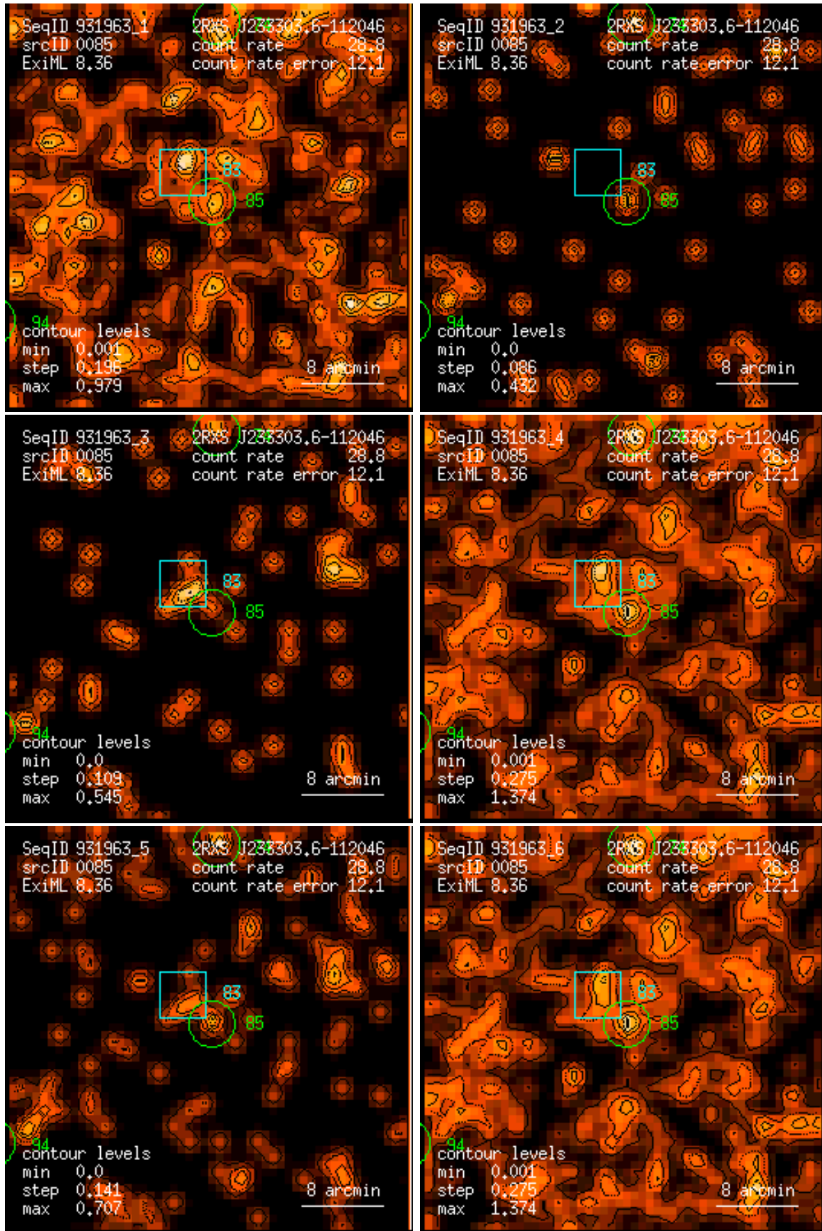
Figure 85: RASS 931963: detection 0085: band rate images, Gaussian filter: (1) PSPC channels 11 – 41, (2) 52 – 90, (3) 91 – 201, (4) 11 – 235, (5) 52 – 201, (6) 11 – 201. Broad band rates in counts/ks. Band rate contour levels in counts/ks/arcmin 2 .
