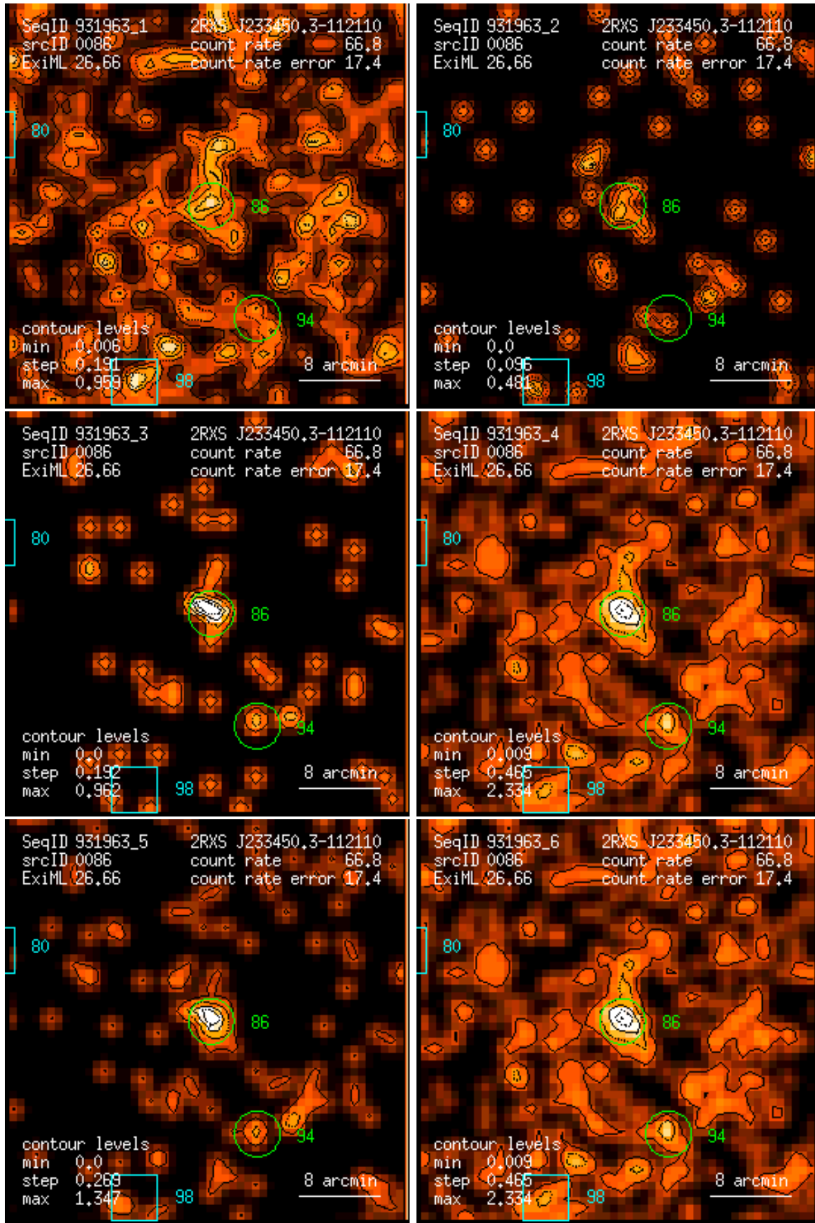
Figure 86: RASS 931963: detection 0086: band rate images, Gaussian filter: (1) PSPC channels 11 – 41, (2) 52 – 90, (3) 91 – 201, (4) 11 – 235, (5) 52 – 201, (6) 11 – 201. Broad band rates in counts/ks. Band rate contour levels in counts/ks/arcmin 2 .
