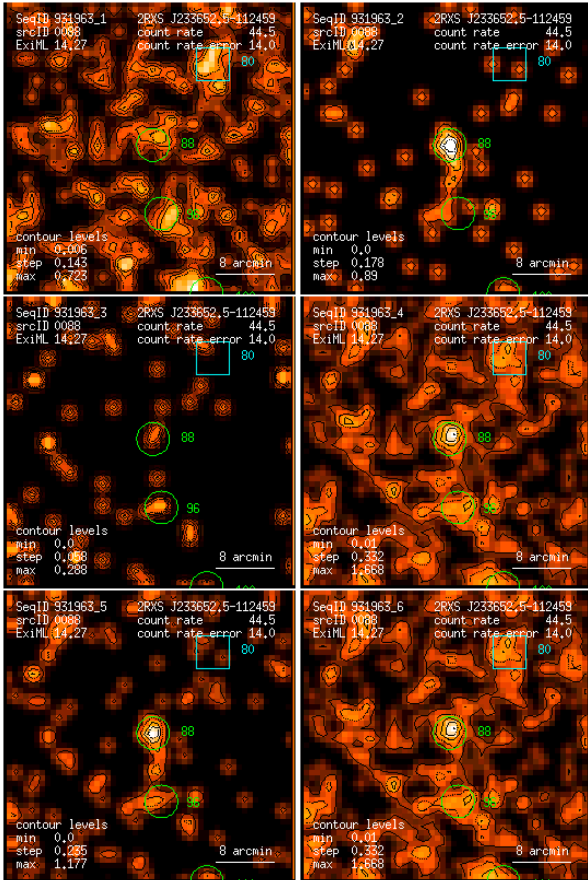
Figure 88: RASS 931963: detection 0088: band rate images, Gaussian filter: (1) PSPC channels 11 – 41, (2) 52 – 90, (3) 91 – 201, (4) 11 – 235, (5) 52 – 201, (6) 11 – 201. Broad band rates in counts/ks. Band rate contour levels in counts/ks/arcmin 2 .
