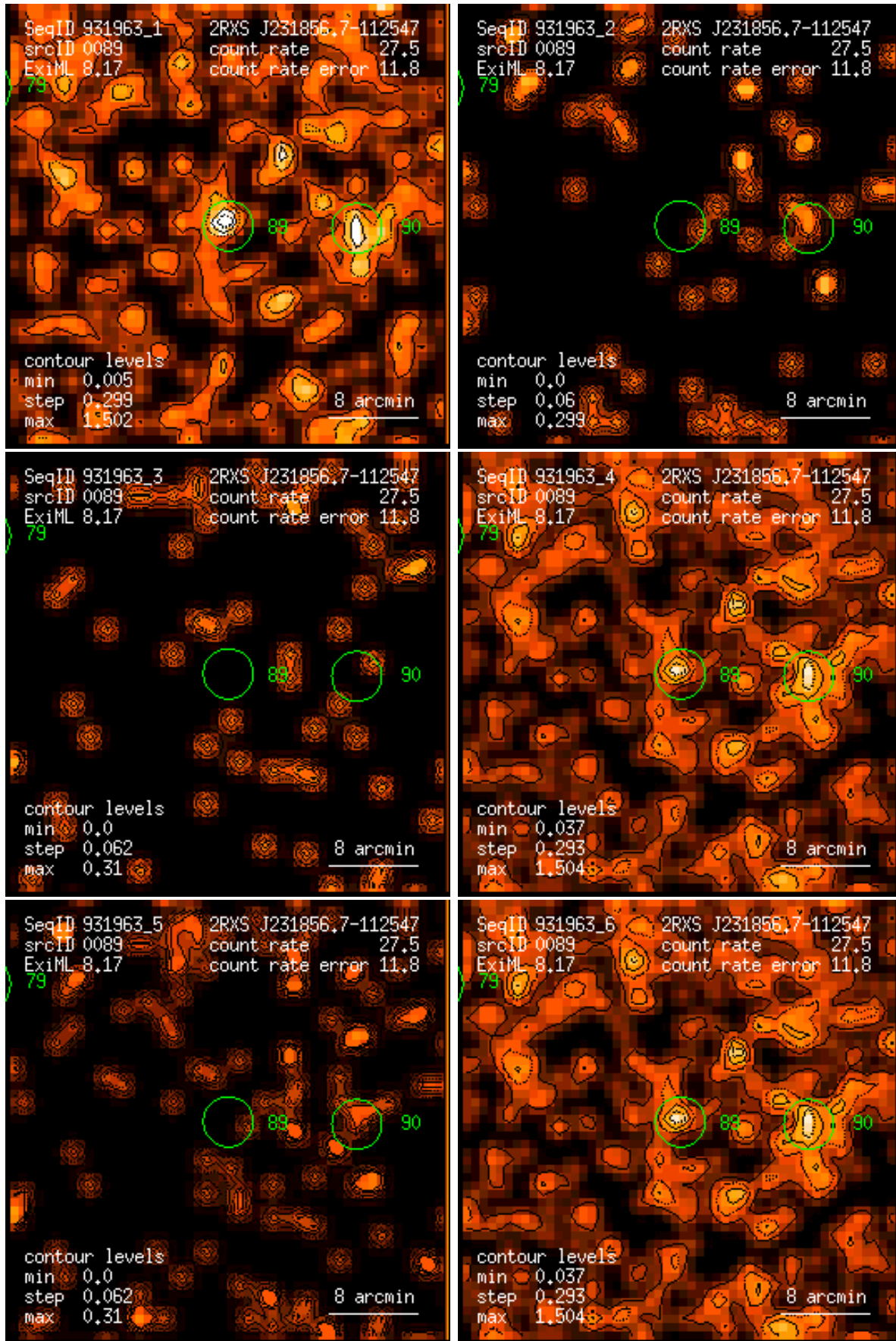
Figure 89: RASS 931963: detection 0089: band rate images, Gaussian filter: (1) PSPC channels 11 – 41, (2) 52 – 90, (3) 91 – 201, (4) 11 – 235, (5) 52 – 201, (6) 11 – 201. Broad band rates in counts/ks. Band rate contour levels in counts/ks/arcmin 2 .
