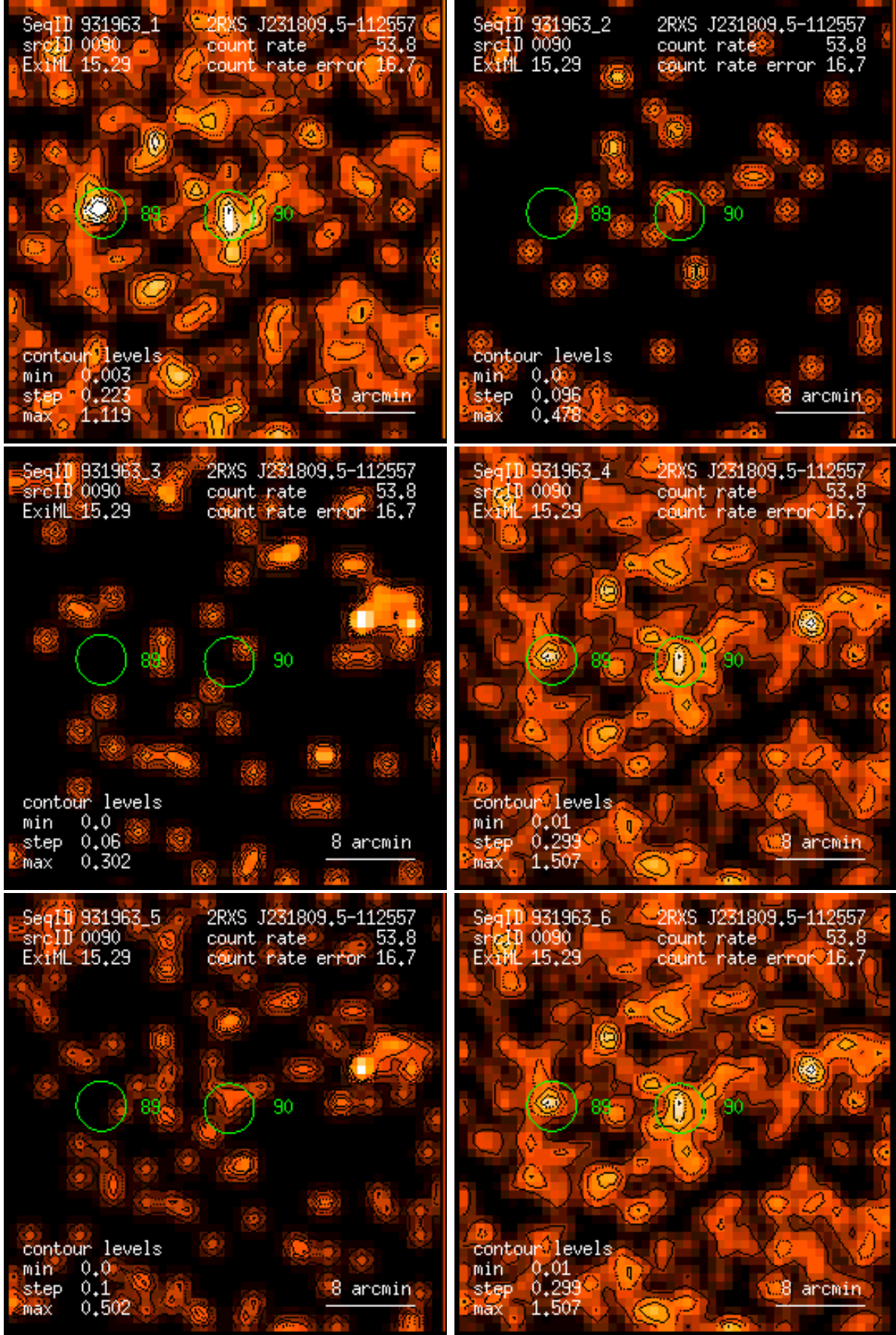
Figure 90: RASS 931963: detection 0090: band rate images, Gaussian filter: (1) PSPC channels 11 – 41, (2) 52 – 90, (3) 91 – 201, (4) 11 – 235, (5) 52 – 201, (6) 11 – 201. Broad band rates in counts/ks. Band rate contour levels in counts/ks/arcmin 2 .
