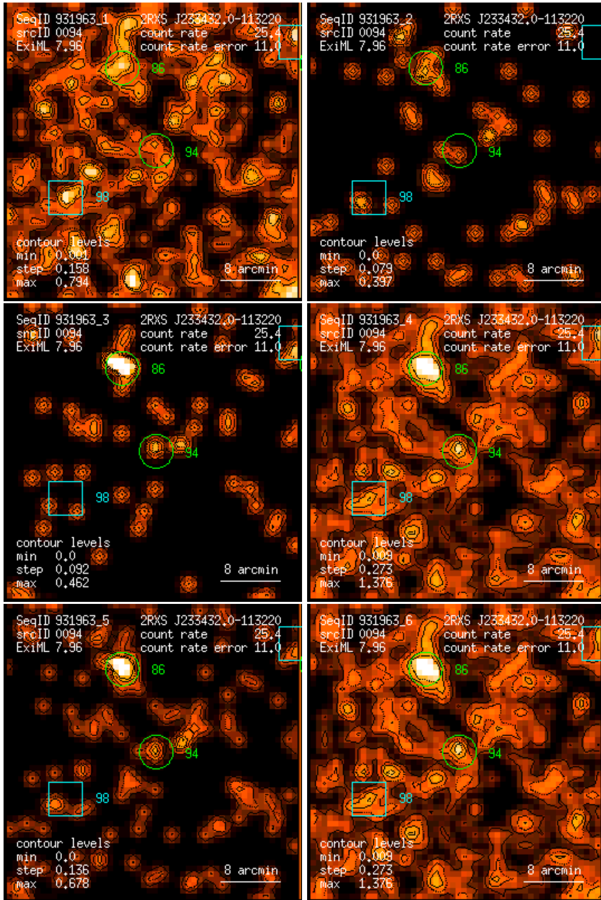
Figure 94: RASS 931963: detection 0094: band rate images, Gaussian filter: (1) PSPC channels 11 – 41, (2) 52 – 90, (3) 91 – 201, (4) 11 – 235, (5) 52 – 201, (6) 11 – 201. Broad band rates in counts/ks. Band rate contour levels in counts/ks/arcmin 2 .
