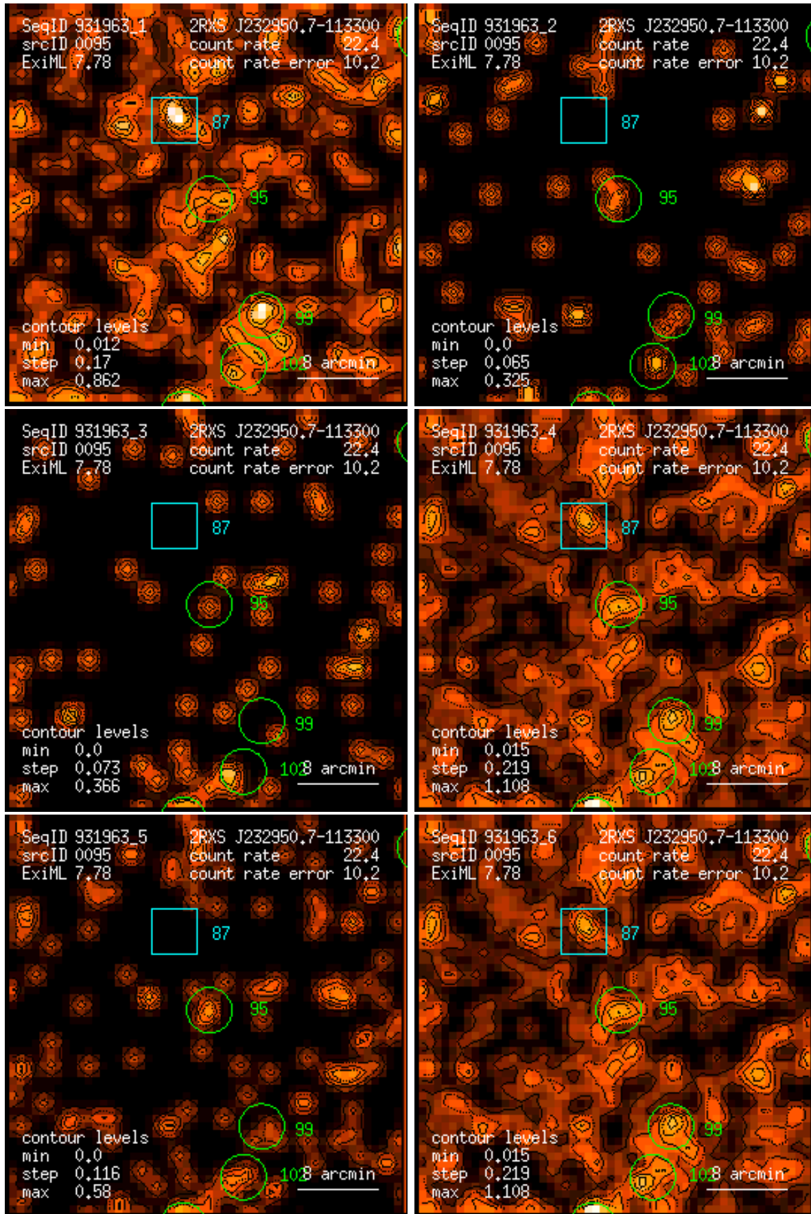
Figure 95: RASS 931963: detection 0095: band rate images, Gaussian filter: (1) PSPC channels 11 – 41, (2) 52 – 90, (3) 91 – 201, (4) 11 – 235, (5) 52 – 201, (6) 11 – 201. Broad band rates in counts/ks. Band rate contour levels in counts/ks/arcmin 2 .
