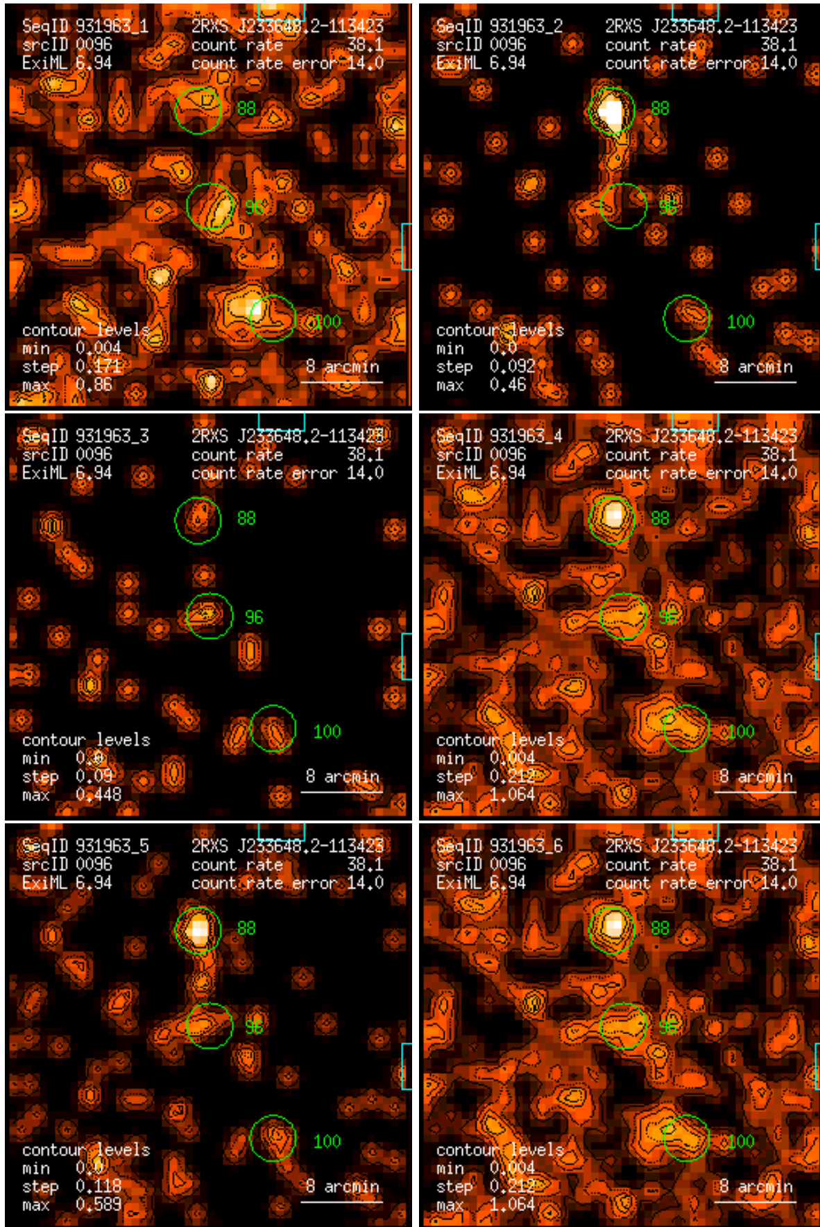
Figure 96: RASS 931963: detection 0096: band rate images, Gaussian filter: (1) PSPC channels 11 – 41, (2) 52 – 90, (3) 91 – 201, (4) 11 – 235, (5) 52 – 201, (6) 11 – 201. Broad band rates in counts/ks. Band rate contour levels in counts/ks/arcmin 2 .
