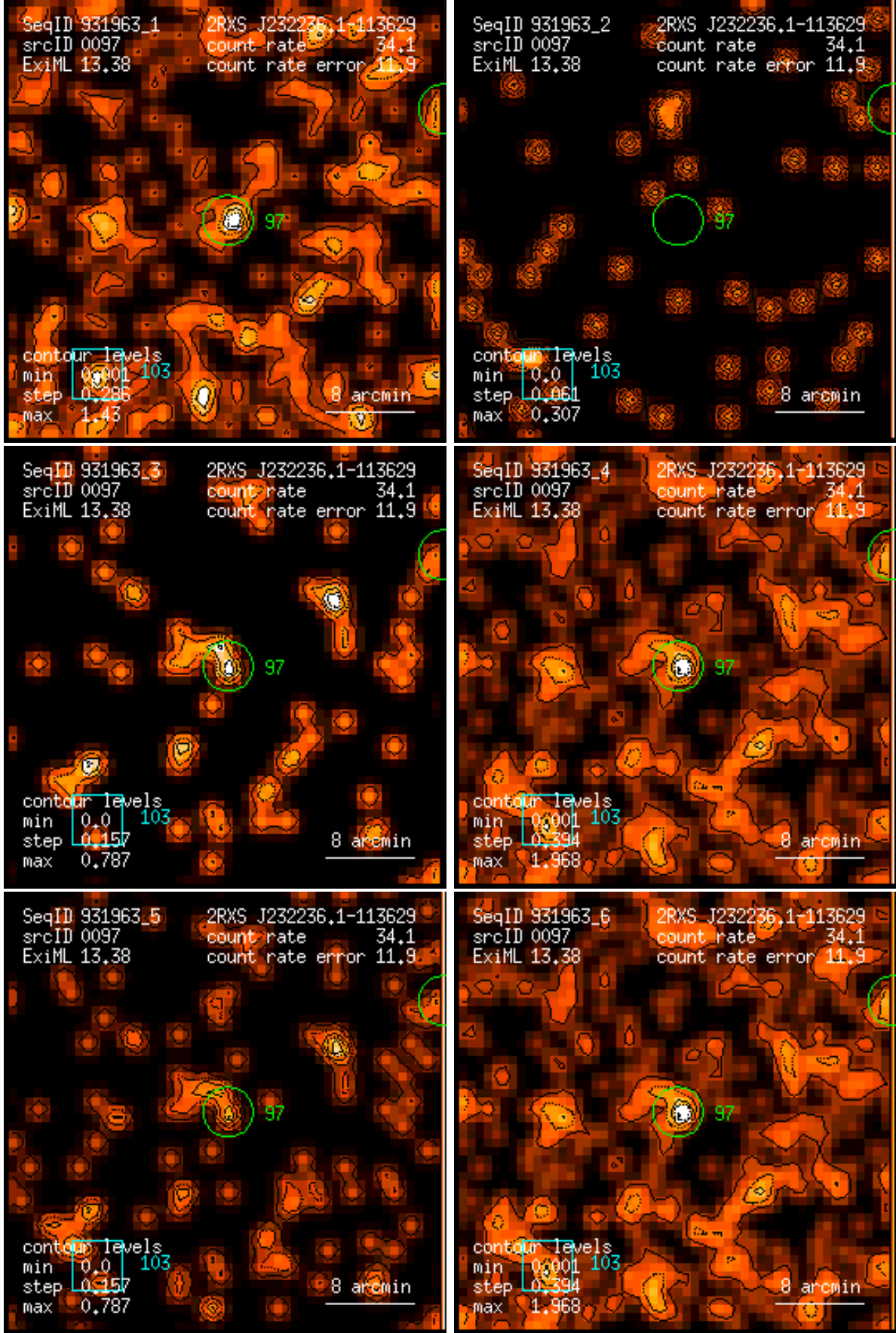
Figure 97: RASS 931963: detection 0097: band rate images, Gaussian filter: (1) PSPP channels 11 – 41, (2) 52 – 90, (3) 91 – 201, (4) 11 – 235, (5) 52 – 201, (6) 11 – 201. Broad band rates in counts/ks. Band rate contour levels in counts/ks/arcmin 2 .
