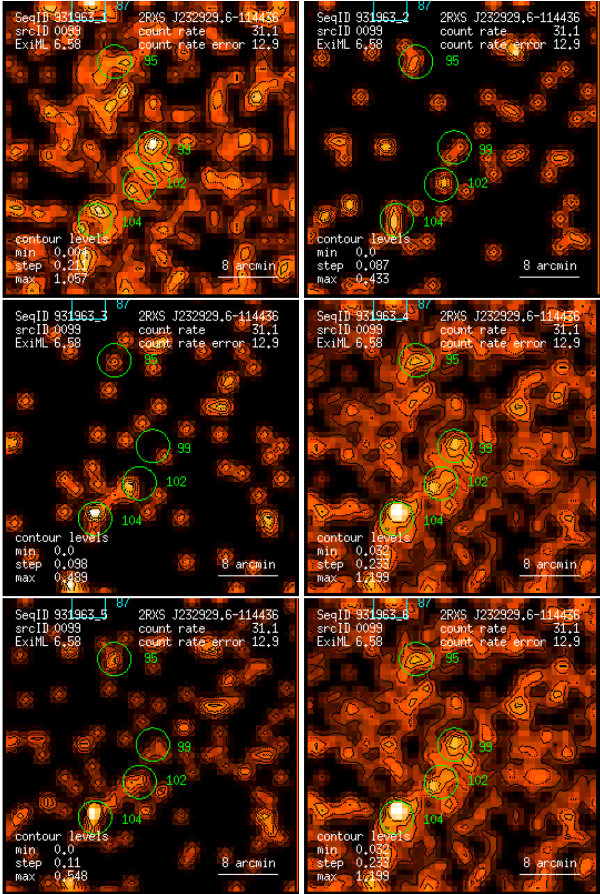
Figure 99: RASS 931963: detection 0099: band rate images, Gaussian filter: (1) PSPC channels 11 – 41, (2) 52 – 90, (3) 91 – 201, (4) 11 – 235, (5) 52 – 201, (6) 11 – 201. Broad band rates in counts/ks. Band rate contour levels in counts/ks/arcmin 2 .
