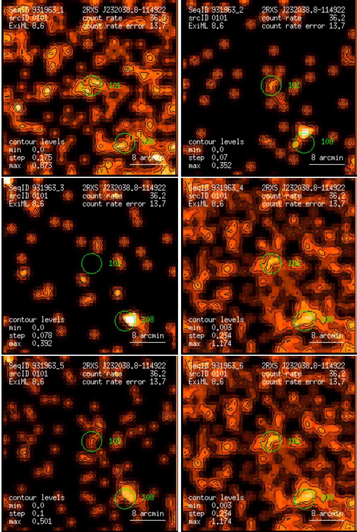
Figure 101: RASS 931963: detection 0101: band rate images, Gaussian filter: (1) PSPC channels 11 – 41, (2) 52 – 90, (3) 91 – 201, (4) 11 – 235, (5) 52 – 201, (6) 11 – 201. Broad band rates in counts/ks. Band rate contour levels in counts/ks/arcmin 2 .
