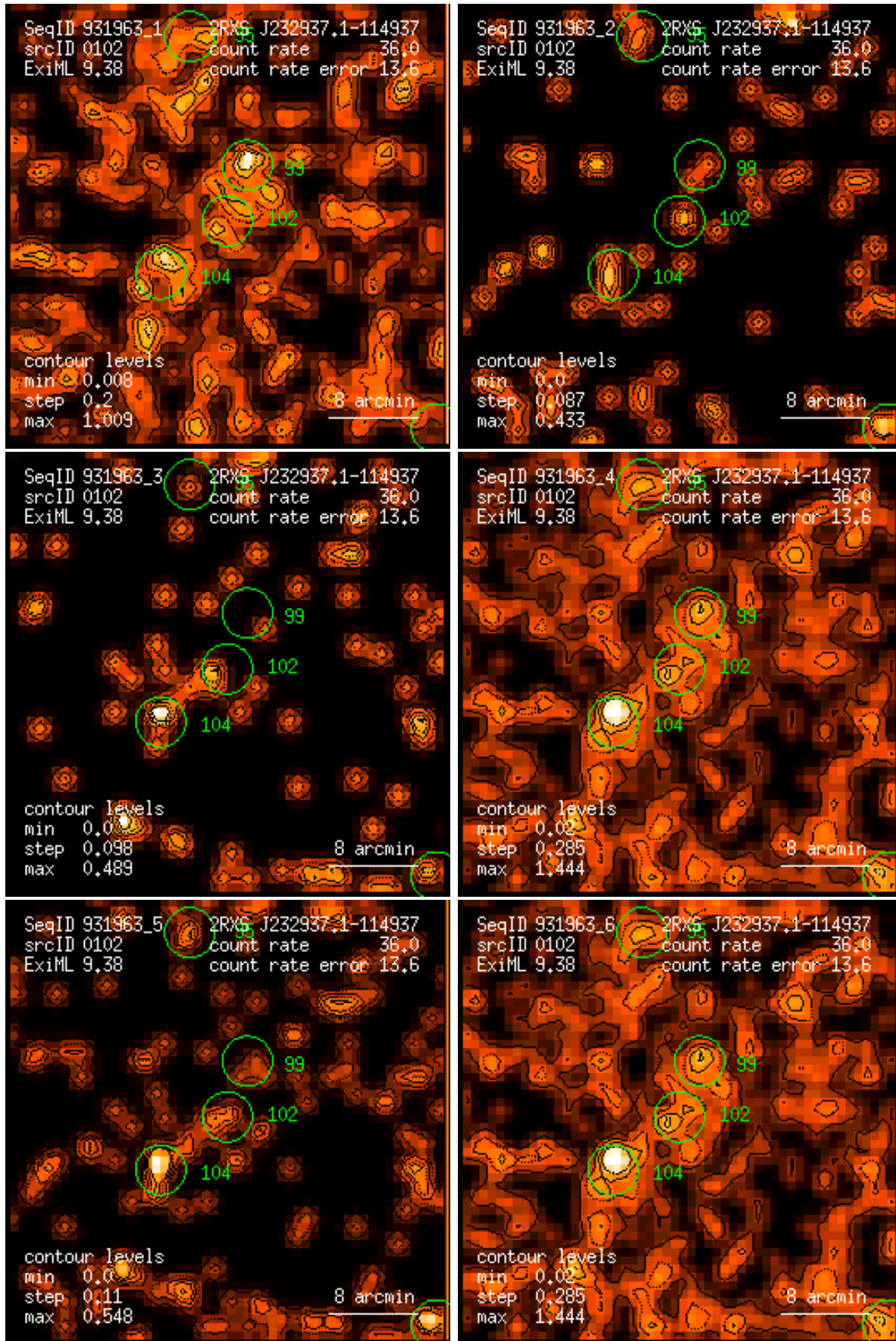
Figure 102: RASS 931963: detection 0102: band rate images, Gaussian filter: (1) PSPC channels 11 – 41, (2) 52 – 90, (3) 91 – 201, (4) 11 – 235, (5) 52 – 201, (6) 11 – 201. Broad band rates in counts/ks. Band rate contour levels in counts/ks/arcmin 2 .
