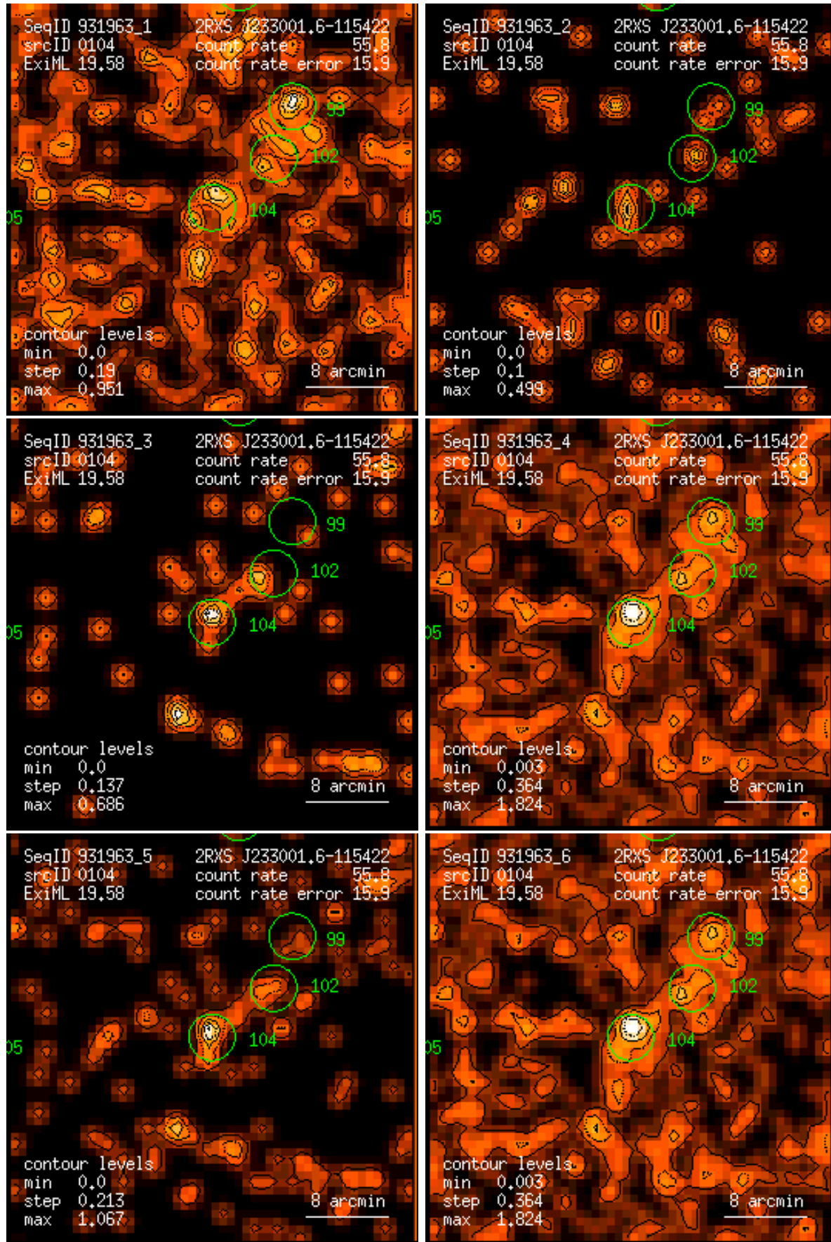
Figure 104: RASS 931963: detection 0104: band rate images, Gaussian filter: (1) PSPC channels 11 – 41, (2) 52 – 90, (3) 91 – 201, (4) 11 – 235, (5) 52 – 201, (6) 11 – 201. Broad band rates in counts/ks. Band rate contour levels in counts/ks/arcmin 2 .
