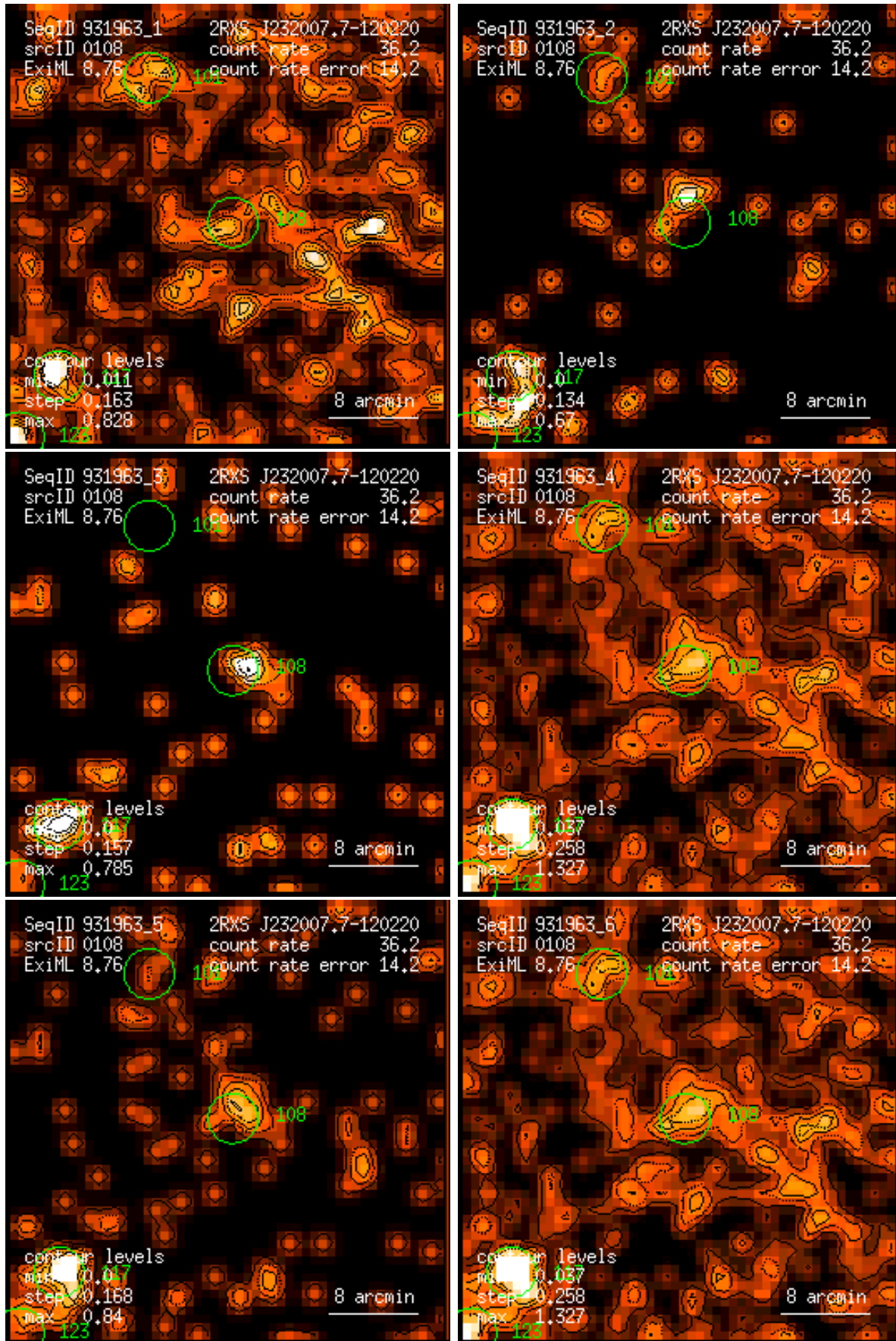
Figure 108: RASS 931963: detection 0108: band rate images, Gaussian filter: (1) PSPC channels 11 – 41, (2) 52 – 90, (3) 91 – 201, (4) 11 – 235, (5) 52 – 201, (6) 11 – 201. Broad band rates in counts/ks. Band rate contour levels in counts/ks/arcmin 2 .
