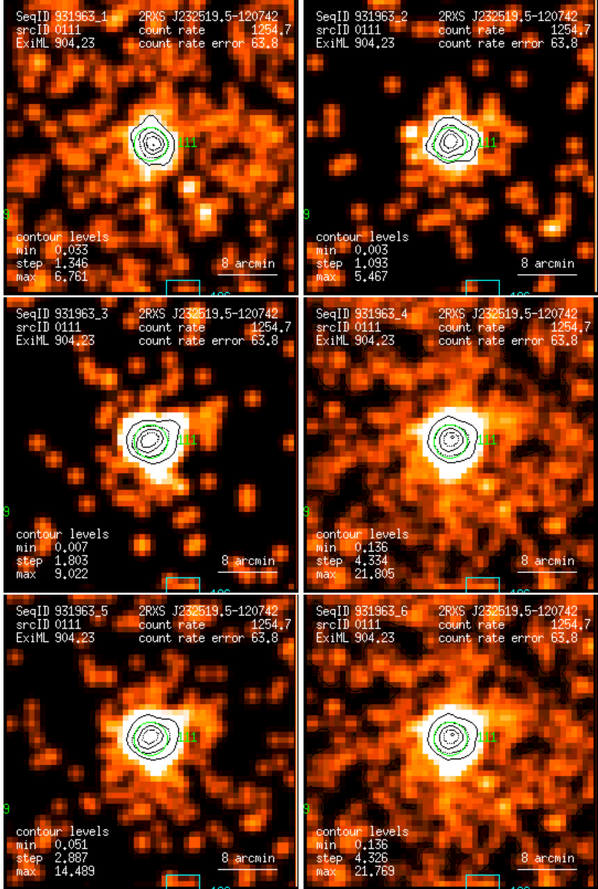
Figure 111: RASS 931963: detection 0111: band rate images, Gaussian filter: (1) PSPC channels 11 – 41, (2) 52 – 90, (3) 91 – 201, (4) 11 – 235, (5) 52 – 201, (6) 11 – 201. Broad band rates in counts/ks. Band rate contour levels in counts/ks/arcmin 2 .
