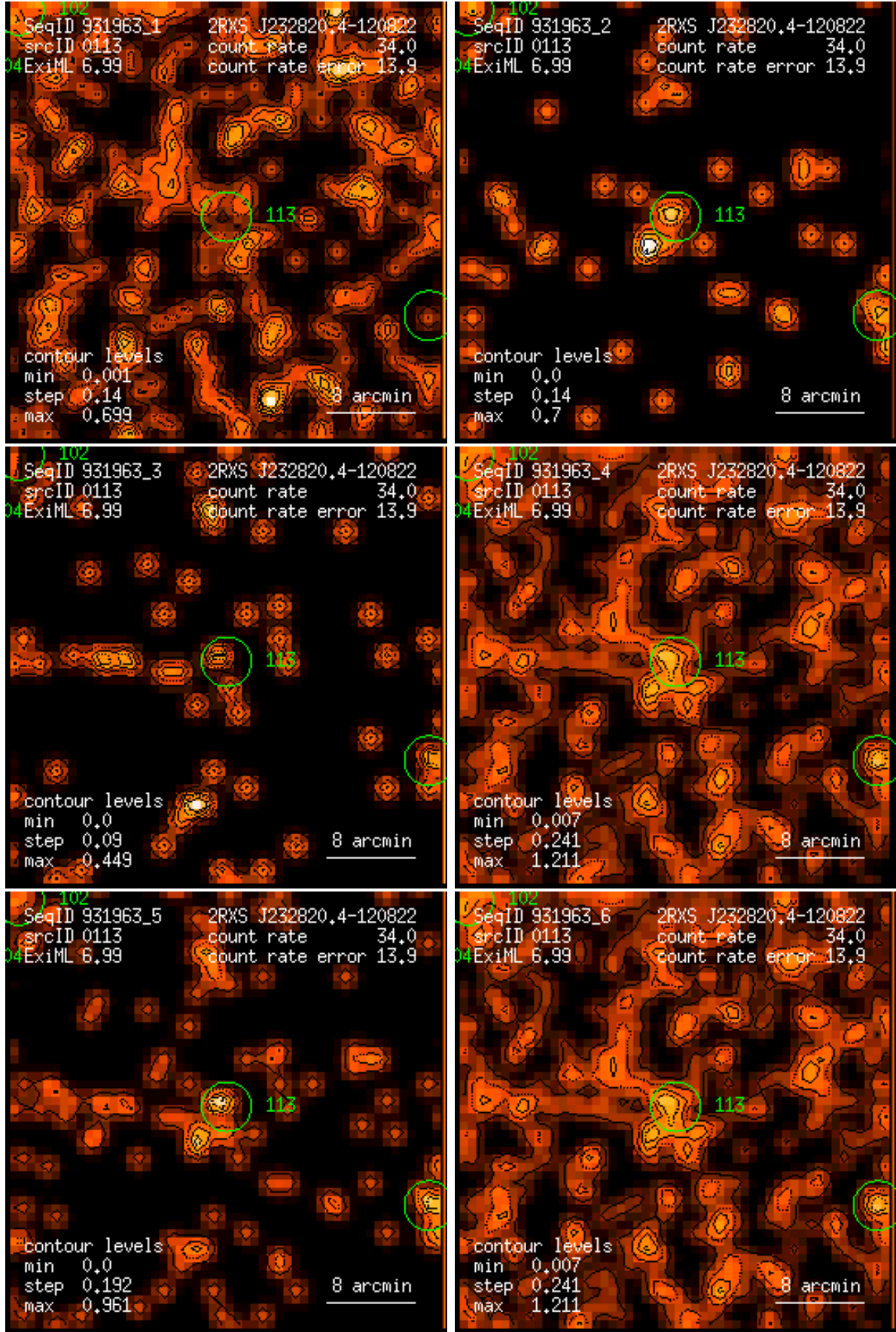
Figure 113: RASS 931963: detection 0113: band rate images, Gaussian filter: (1) PSPC channels 11 – 41, (2) 52 – 90, (3) 91 – 201, (4) 11 – 235, (5) 52 – 201, (6) 11 – 201. Broad band rates in counts/ks. Band rate contour levels in counts/ks/arcmin 2 .
