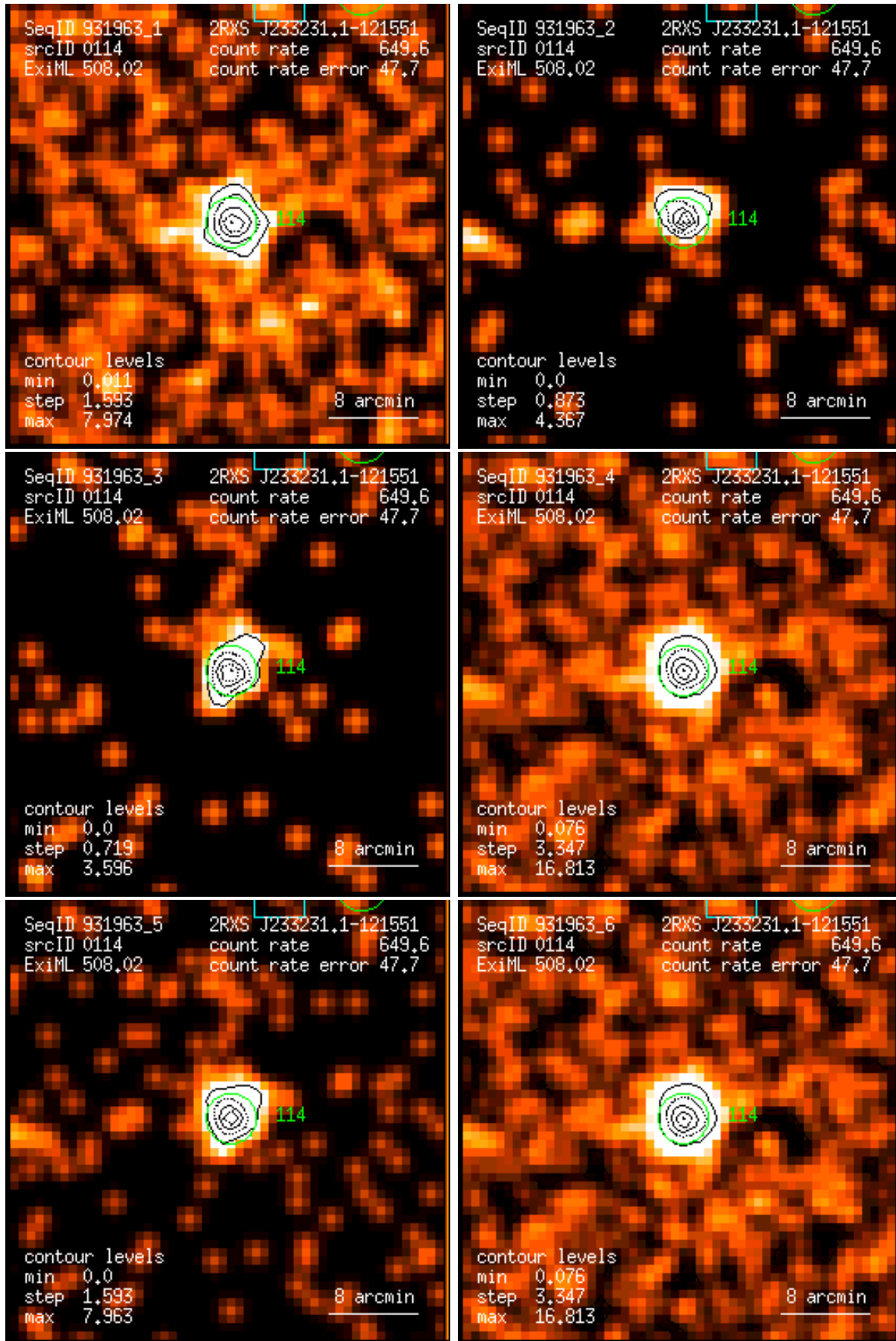
Figure 114: RASS 931963: detection 0114: band rate images, Gaussian filter: (1) PSPC channels 11 – 41, (2) 52 – 90, (3) 91 – 201, (4) 11 – 235, (5) 52 – 201, (6) 11 – 201. Broad band rates in counts/ks. Band rate contour levels in counts/ks/arcmin 2 .
