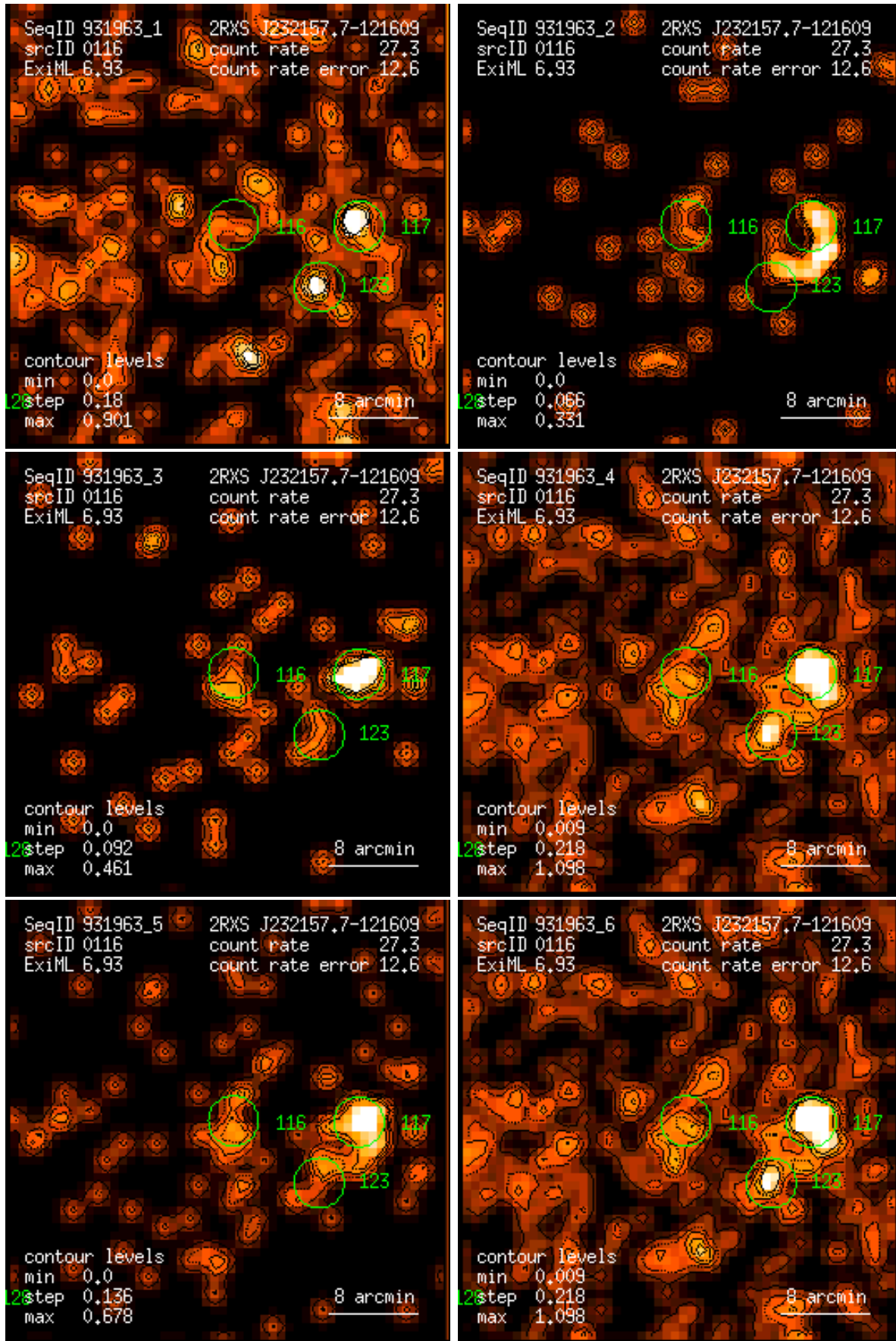
Figure 116: RASS 931963: detection 0116: band rate images, Gaussian filter: (1) PSPC channels 11 – 41, (2) 52 – 90, (3) 91 – 201, (4) 11 – 235, (5) 52 – 201, (6) 11 – 201. Broad band rates in counts/ks. Band rate contour levels in counts/ks/arcmin 2 .
