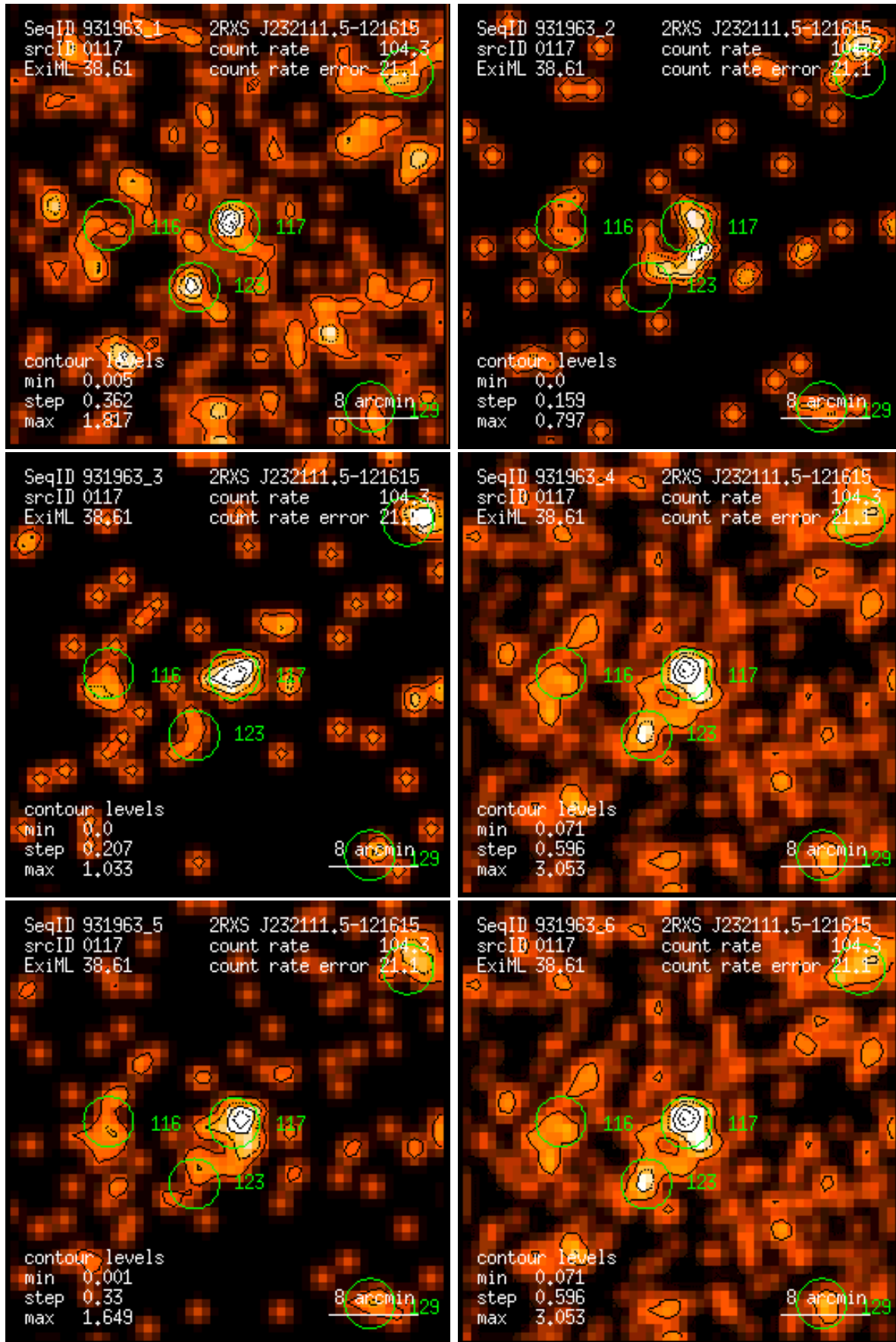
Figure 117: RASS 931963: detection 0117: band rate images, Gaussian filter: (1) PSPC channels 11 – 41, (2) 52 – 90, (3) 91 – 201, (4) 11 – 235, (5) 52 – 201, (6) 11 – 201. Broad band rates in counts/ks. Band rate contour levels in counts/ks/arcmin 2 .
