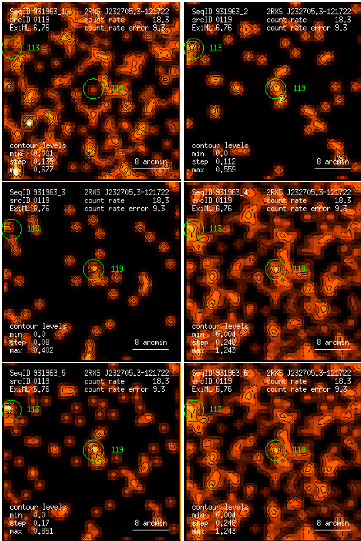
Figure 119: RASS 931963: detection 0119: band rate images, Gaussian filter: (1) PSPC channels 11 – 41, (2) 52 – 90, (3) 91 – 201, (4) 11 – 235, (5) 52 – 201, (6) 11 – 201. Broad band rates in counts/ks. Band rate contour levels in counts/ks/arcmin 2 .
