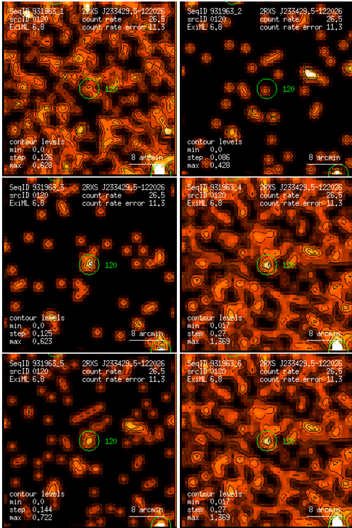
Figure 120: RASS 931963: detection 0120: band rate images, Gaussian filter: (1) PSPC channels 11 – 41, (2) 52 – 90, (3) 91 – 201, (4) 11 – 235, (5) 52 – 201, (6) 11 – 201. Broad band rates in counts/ks. Band rate contour levels in counts/ks/arcmin 2 .
