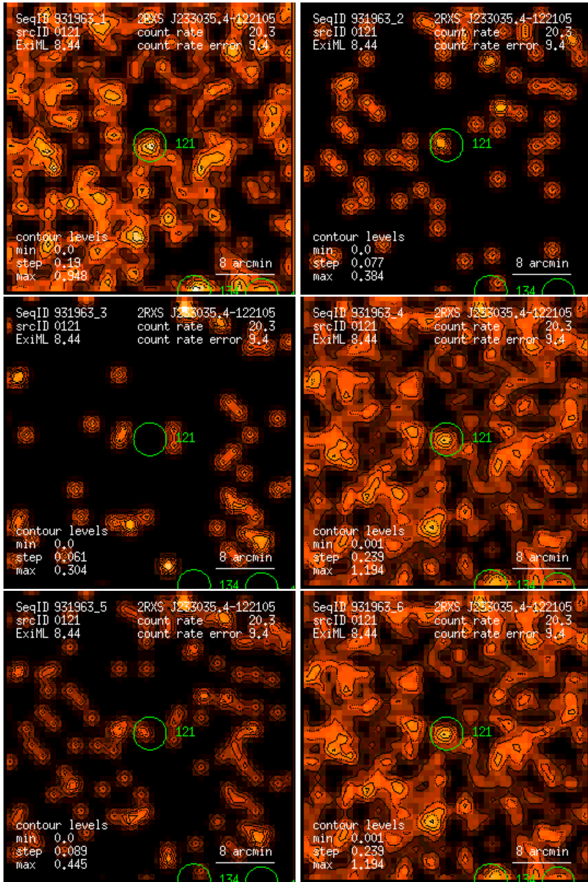
Figure 121: RASS 931963: detection 0121: band rate images, Gaussian filter: (1) PSPC channels 11 – 41, (2) 52 – 90, (3) 91 – 201, (4) 11 – 235, (5) 52 – 201, (6) 11 – 201. Broad band rates in counts/ks. Band rate contour levels in counts/ks/arcmin 2 .
