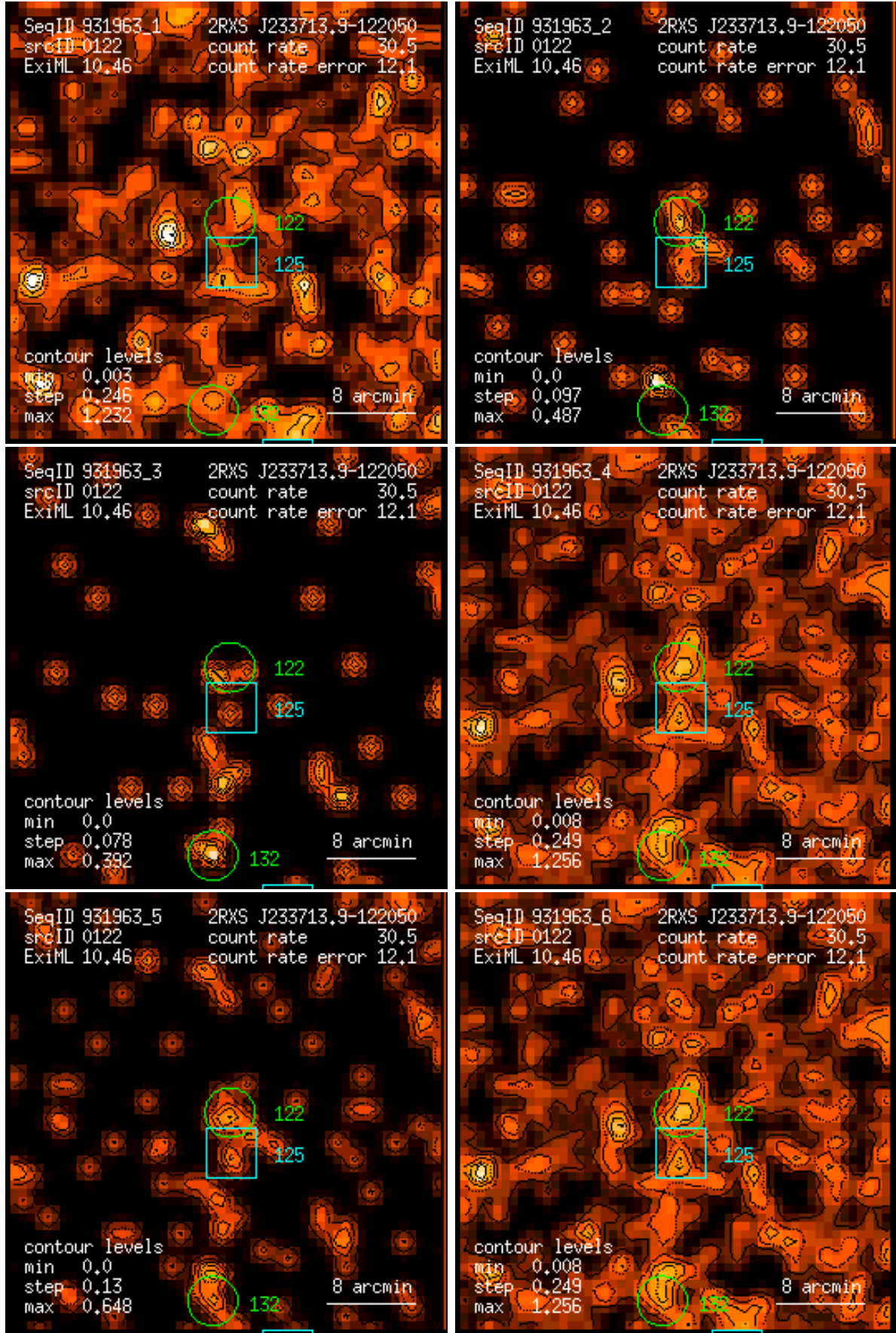
Figure 122: RASS 931963: detection 0122: band rate images, Gaussian filter: (1) PSPC channels 11 – 41, (2) 52 – 90, (3) 91 – 201, (4) 11 – 235, (5) 52 – 201, (6) 11 – 201. Broad band rates in counts/ks. Band rate contour levels in counts/ks/arcmin 2 .
