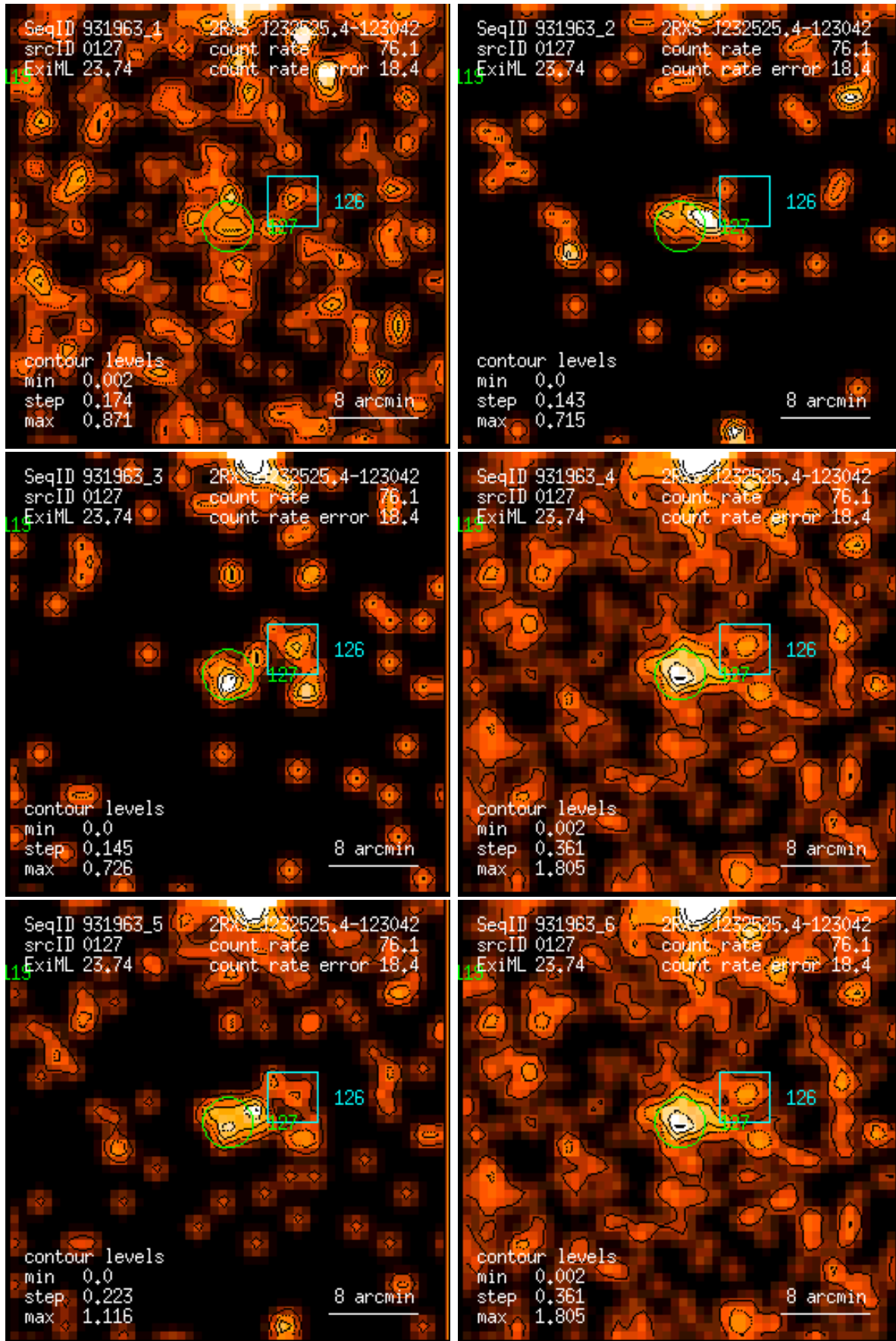
Figure 127: RASS 931963: detection 0127: band rate images, Gaussian filter: (1) PSPC channels 11 – 41, (2) 52 – 90, (3) 91 – 201, (4) 11 – 235, (5) 52 – 201, (6) 11 – 201. Broad band rates in counts/ks. Band rate contour levels in counts/ks/arcmin 2 .
