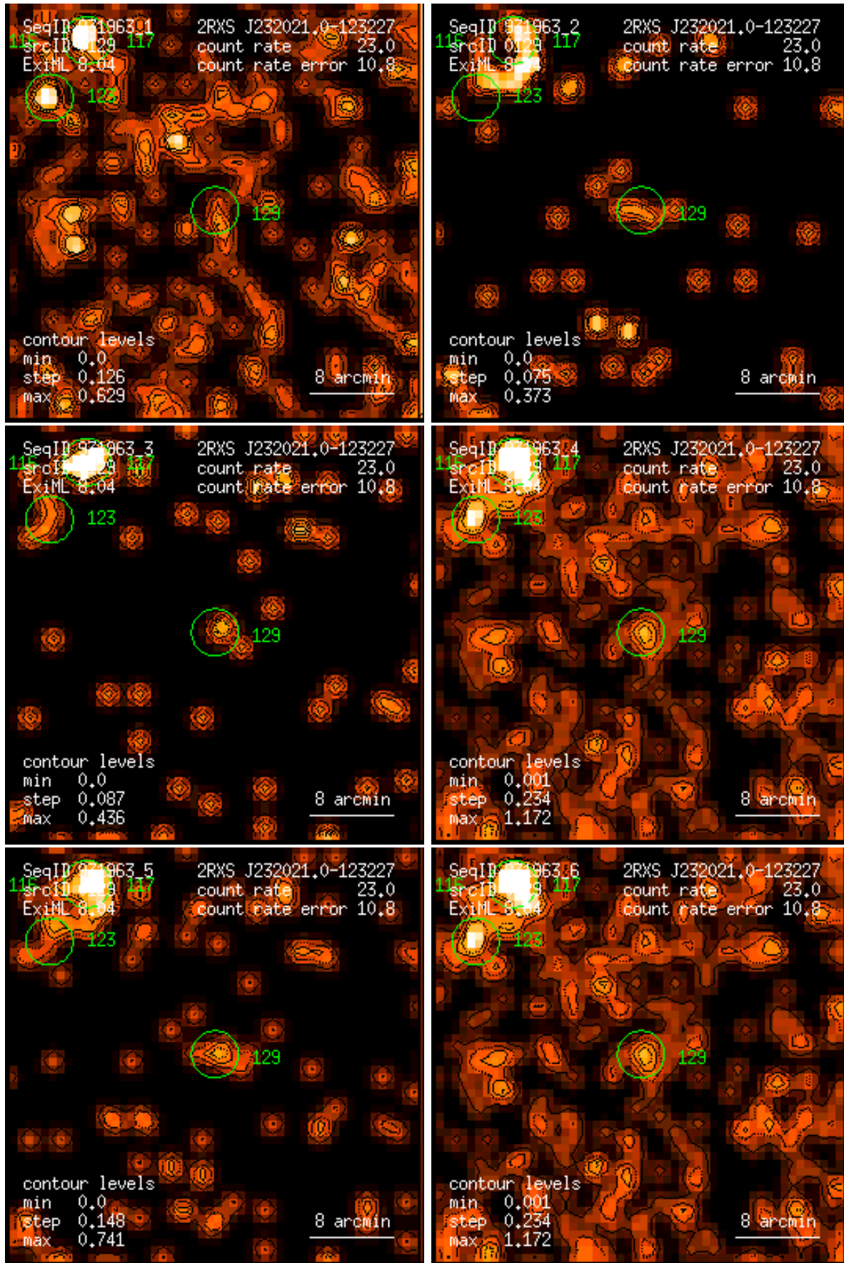
Figure 129: RASS 931963: detection 0129: band rate images, Gaussian filter: (1) PSPC channels 11 – 41, (2) 52 – 90, (3) 91 – 201, (4) 11 – 235, (5) 52 – 201, (6) 11 – 201. Broad band rates in counts/ks. Band rate contour levels in counts/ks/arcmin 2 .
