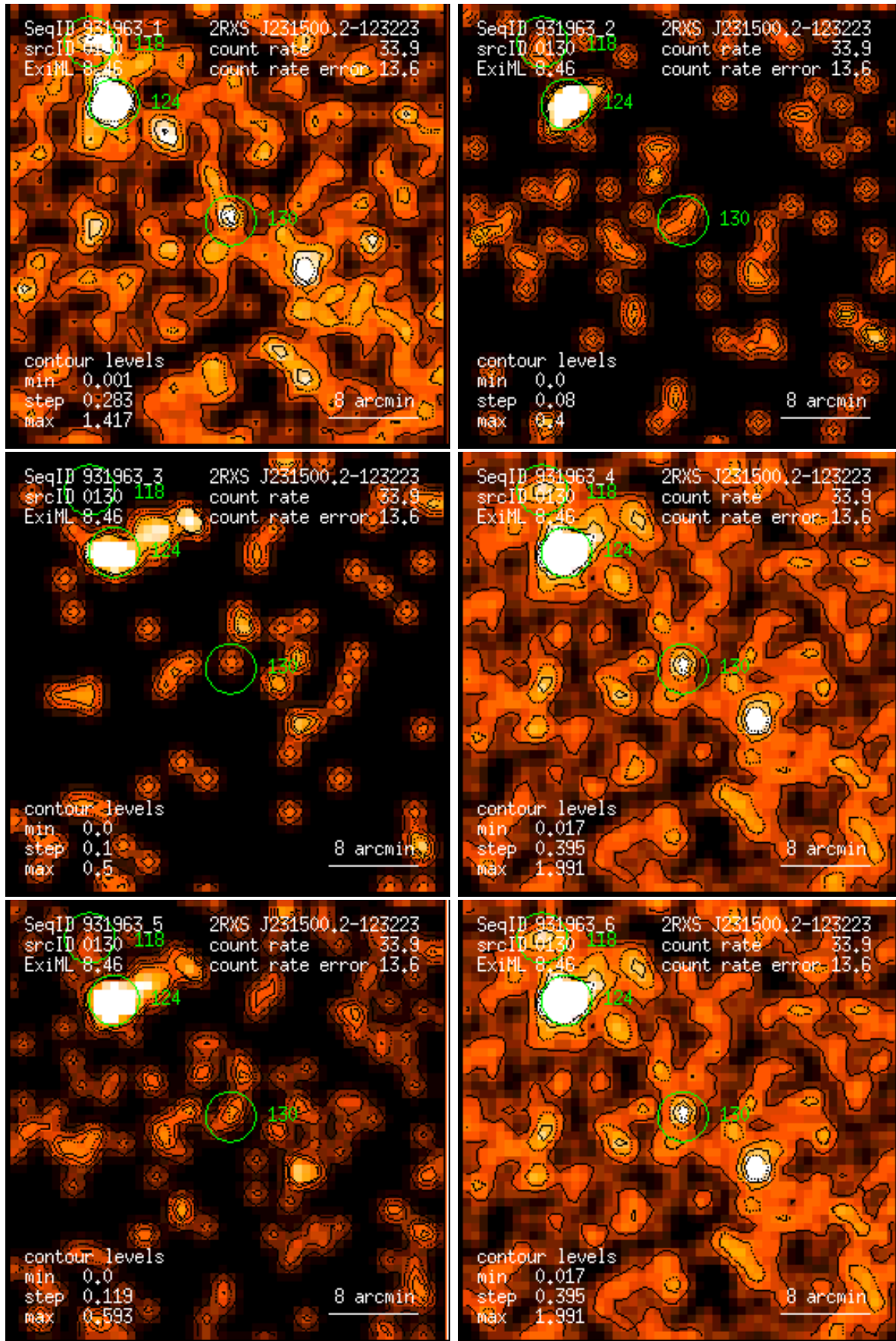
Figure 130: RASS 931963: detection 0130: band rate images, Gaussian filter: (1) PSPC channels 11 – 41, (2) 52 – 90, (3) 91 – 201, (4) 11 – 235, (5) 52 – 201, (6) 11 – 201. Broad band rates in counts/ks. Band rate contour levels in counts/ks/arcmin 2 .
