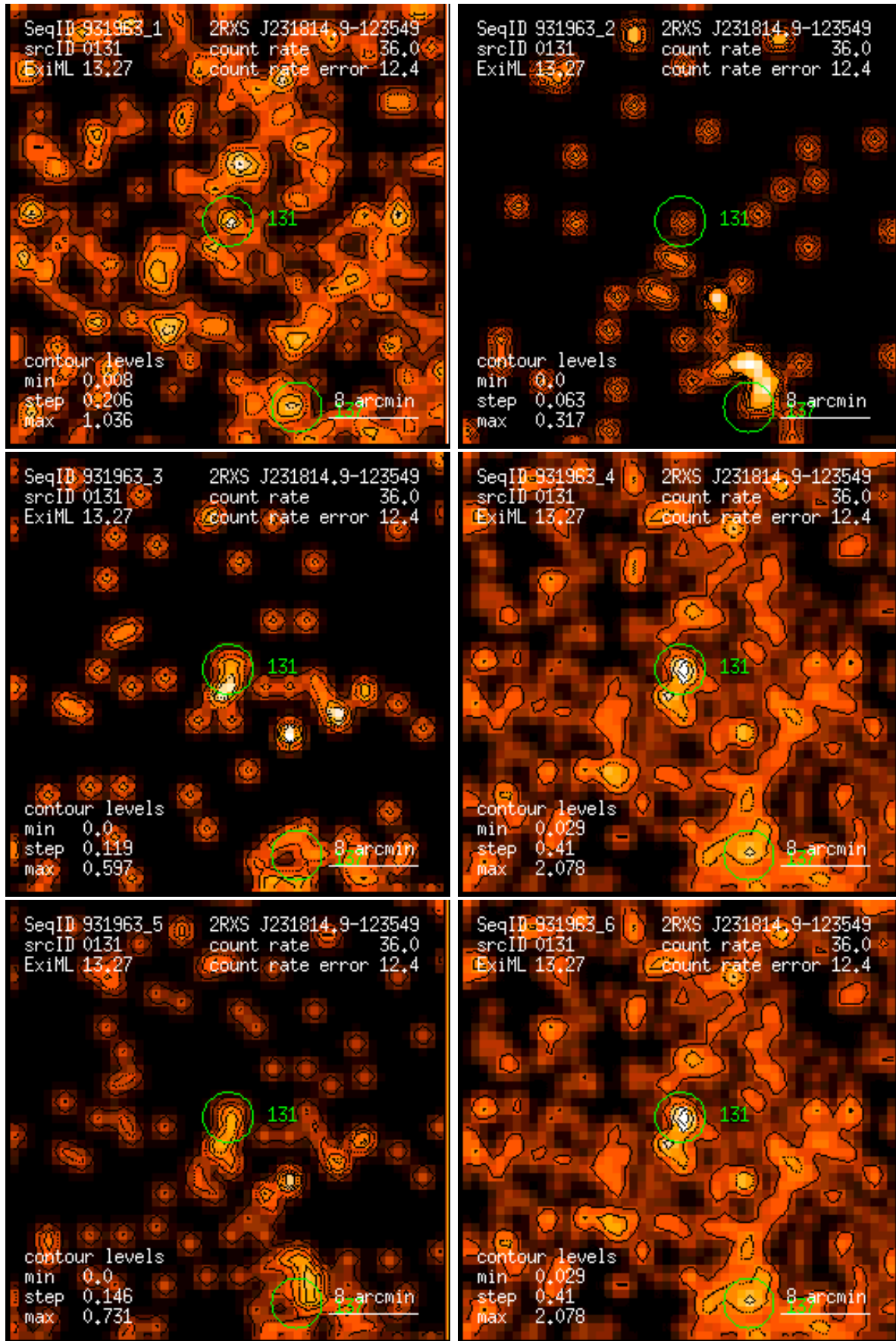
Figure 131: RASS 931963: detection 0131: band rate images, Gaussian filter: (1) PSPC channels 11 – 41, (2) 52 – 90, (3) 91 – 201, (4) 11 – 235, (5) 52 – 201, (6) 11 – 201. Broad band rates in counts/ks. Band rate contour levels in counts/ks/arcmin 2 .
