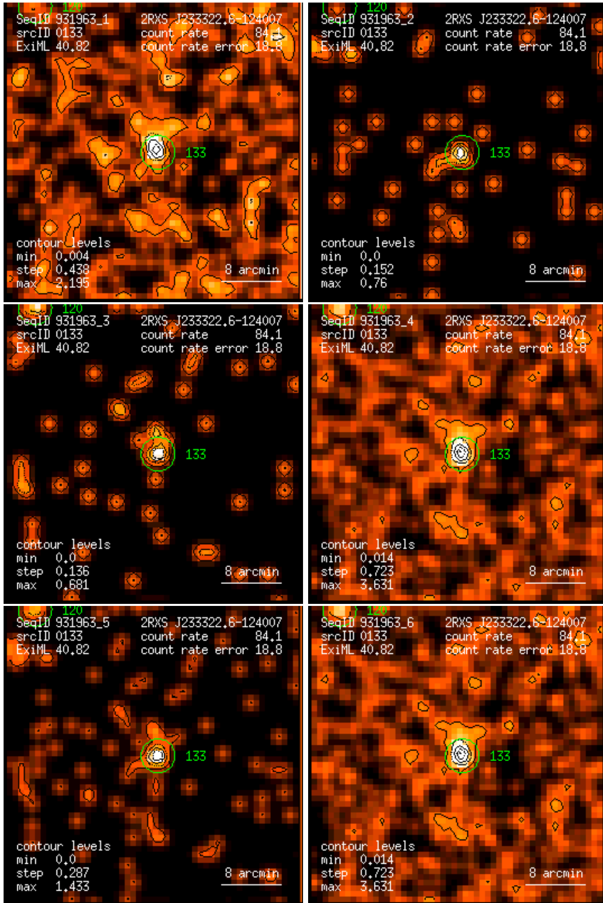
Figure 133: RASS 931963: detection 0133: band rate images, Gaussian filter: (1) PSPC channels 11 – 41, (2) 52 – 90, (3) 91 – 201, (4) 11 – 235, (5) 52 – 201, (6) 11 – 201. Broad band rates in counts/ks. Band rate contour levels in counts/ks/arcmin 2 .
