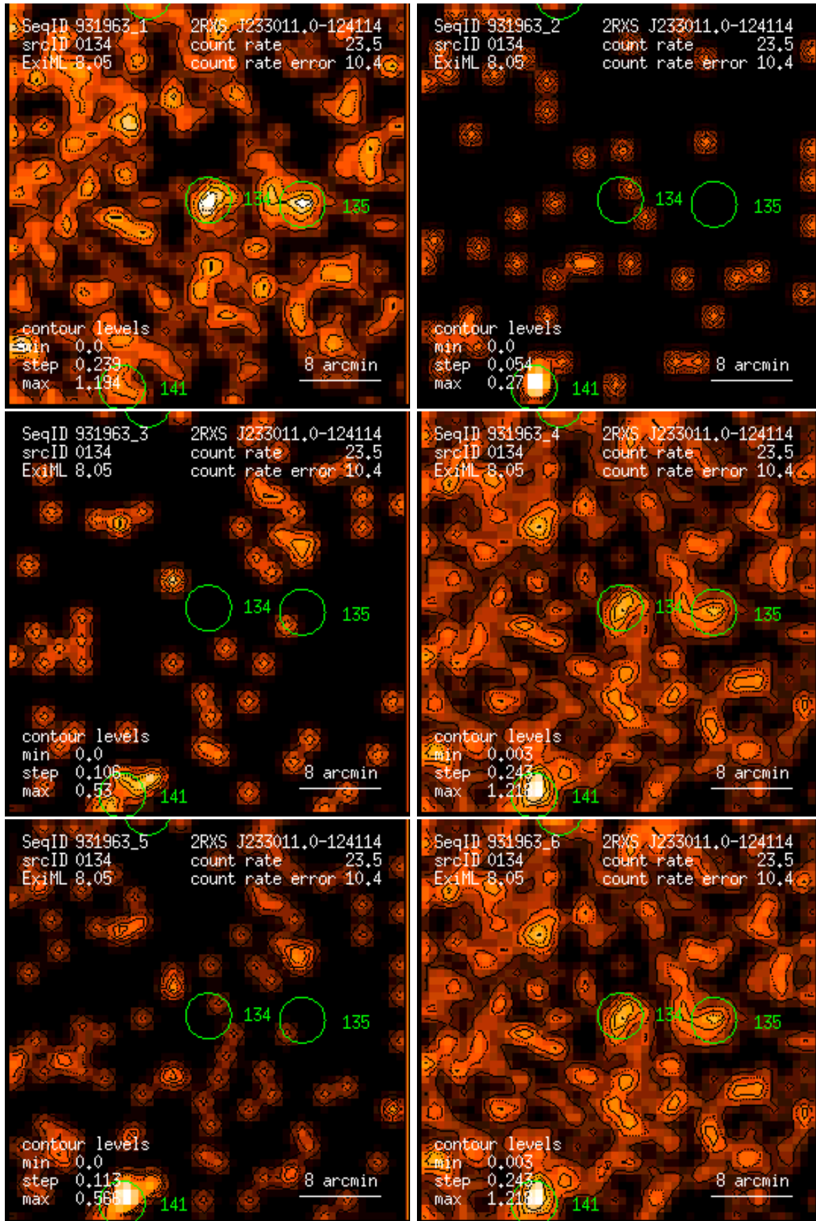
Figure 134: RASS 931963: detection 0134: band rate images, Gaussian filter: (1) PSPC channels 11 – 41, (2) 52 – 90, (3) 91 – 201, (4) 11 – 235, (5) 52 – 201, (6) 11 – 201. Broad band rates in counts/ks. Band rate contour levels in counts/ks/arcmin 2 .
