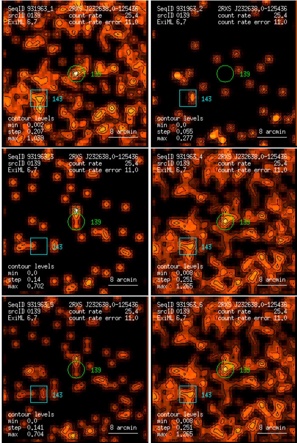
Figure 139: RASS 931963: detection 0139: band rate images, Gaussian filter: (1) PSPC channels 11 – 41, (2) 52 – 90, (3) 91 – 201, (4) 11 – 235, (5) 52 – 201, (6) 11 – 201. Broad band rates in counts/ks. Band rate contour levels in counts/ks/arcmin 2 .
