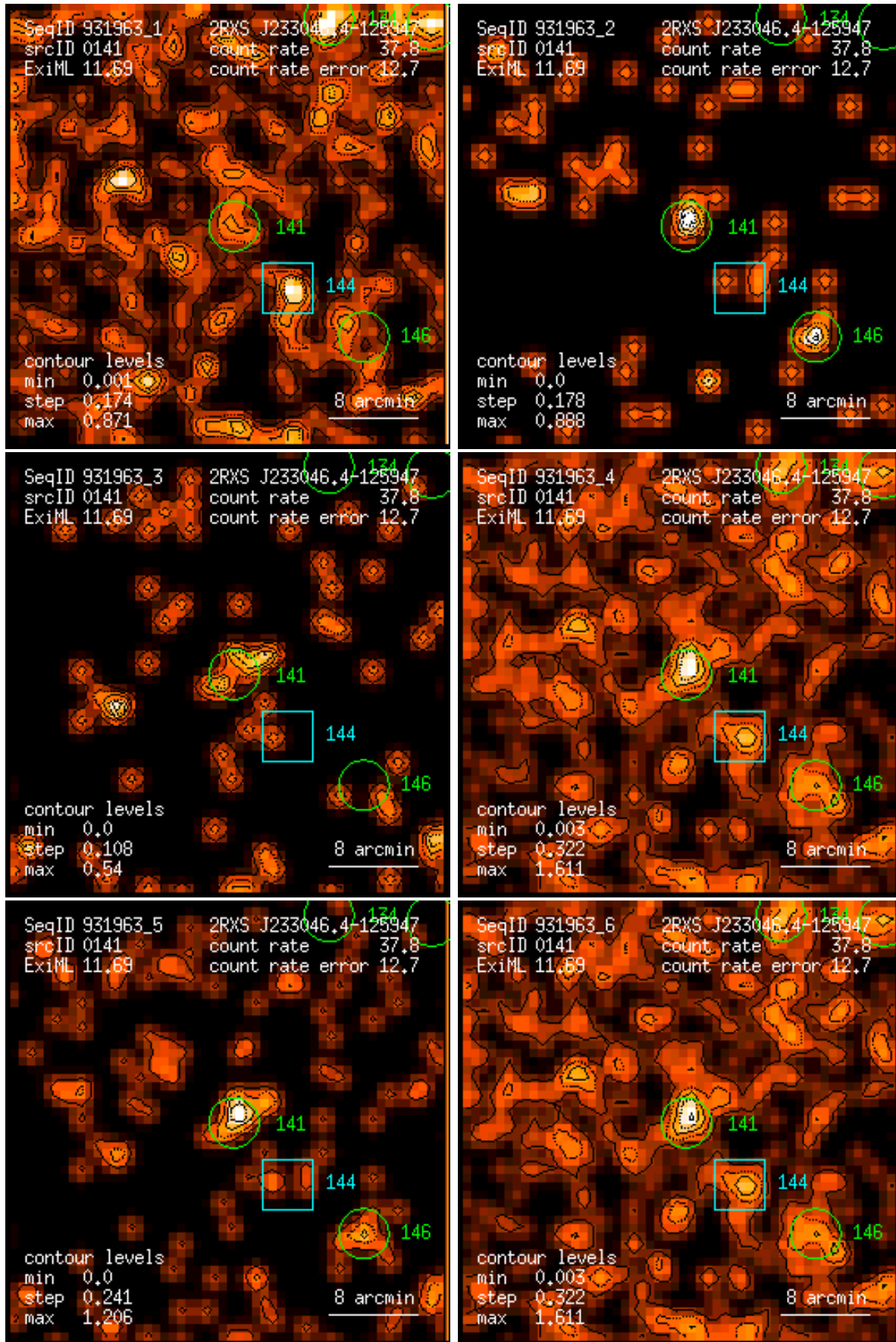
Figure 141: RASS 931963: detection 0141: band rate images, Gaussian filter: (1) PSPC channels 11 – 41, (2) 52 – 90, (3) 91 – 201, (4) 11 – 235, (5) 52 – 201, (6) 11 – 201. Broad band rates in counts/ks. Band rate contour levels in counts/ks/arcmin 2 .
