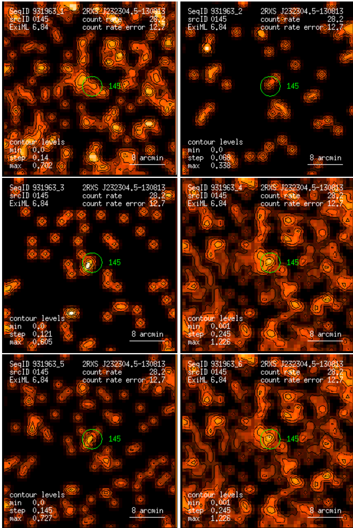
Figure 145: RASS 931963: detection 0145: band rate images, Gaussian filter: (1) PSPC channels 11 – 41, (2) 52 – 90, (3) 91 – 201, (4) 11 – 235, (5) 52 – 201, (6) 11 – 201. Broad band rates in counts/ks. Band rate contour levels in counts/ks/arcmin 2 .
