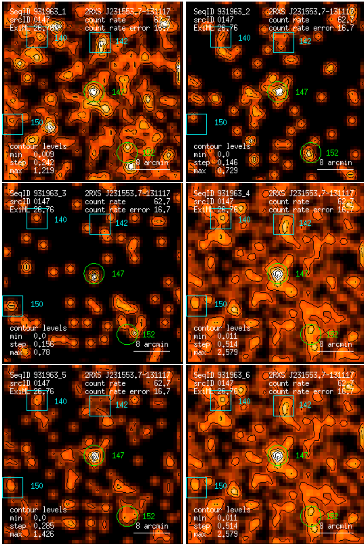
Figure 147: RASS 931963: detection 0147: band rate images, Gaussian filter: (1) PSPC channels 11 – 41, (2) 52 – 90, (3) 91 – 201, (4) 11 – 235, (5) 52 – 201, (6) 11 – 201. Broad band rates in counts/ks. Band rate contour levels in counts/ks/arcmin 2 .
