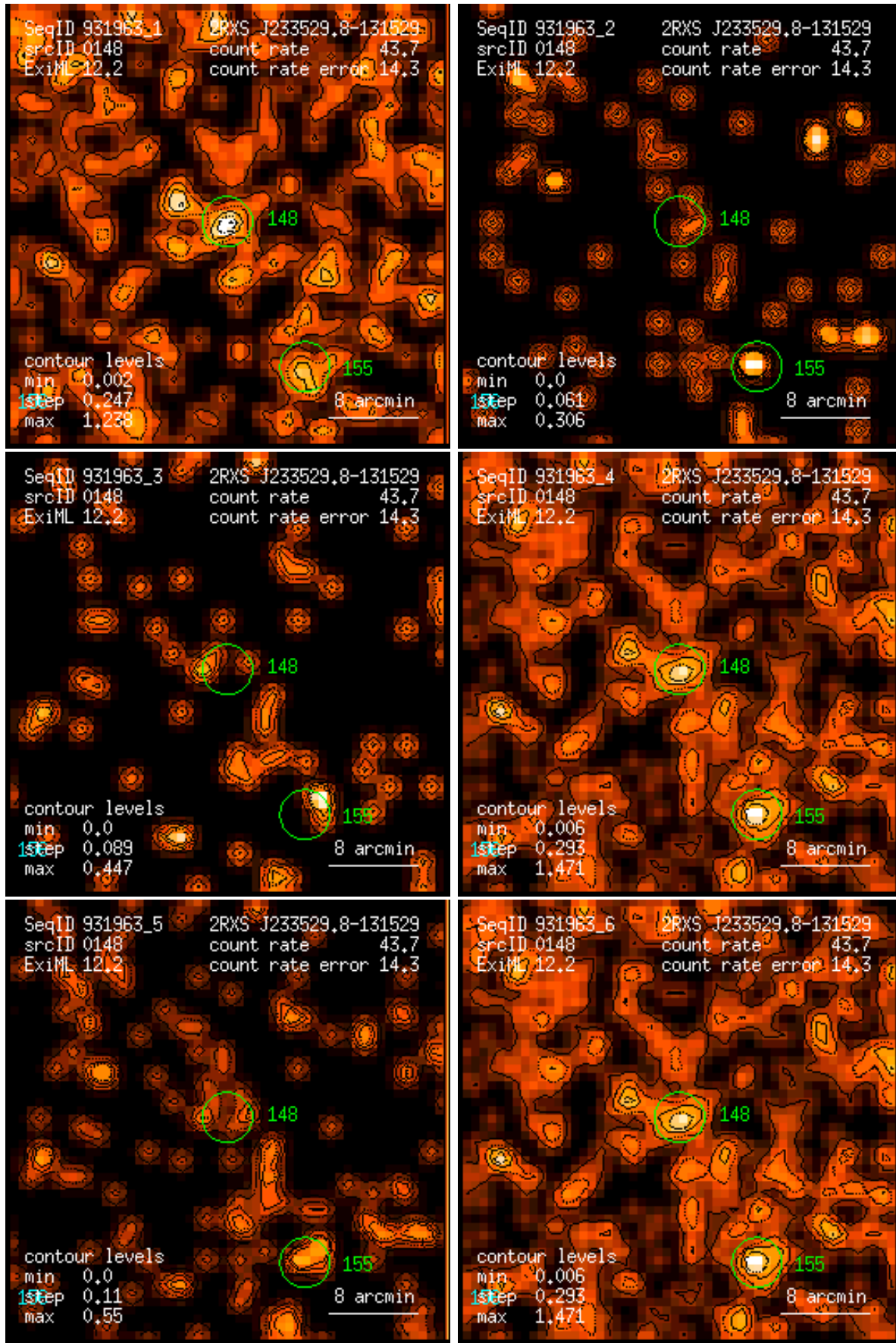
Figure 148: RASS 931963: detection 0148: band rate images, Gaussian filter: (1) PSPC channels 11 – 41, (2) 52 – 90, (3) 91 – 201, (4) 11 – 235, (5) 52 – 201, (6) 11 – 201. Broad band rates in counts/ks. Band rate contour levels in counts/ks/arcmin 2 .
