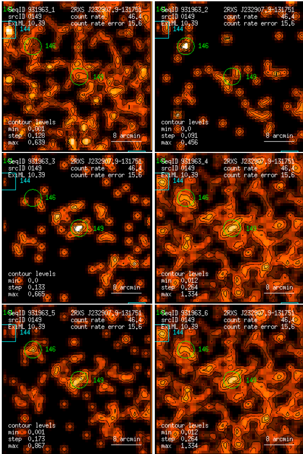
Figure 149: RASS 931963: detection 0149: band rate images, Gaussian filter: (1) PSPC channels 11 – 41, (2) 52 – 90, (3) 91 – 201, (4) 11 – 235, (5) 52 – 201, (6) 11 – 201. Broad band rates in counts/ks. Band rate contour levels in counts/ks/arcmin 2 .
