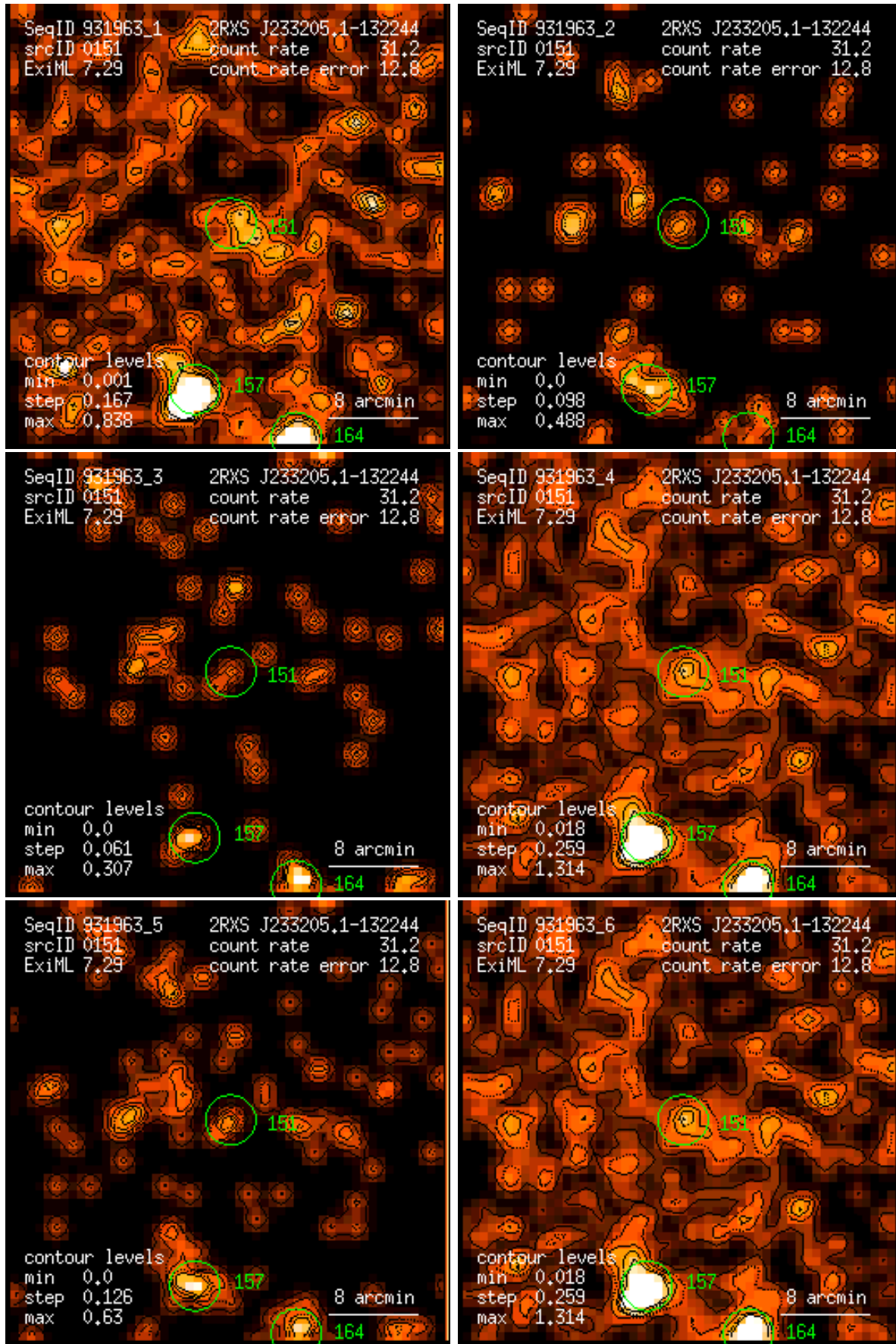
Figure 151: RASS 931963: detection 0151: band rate images, Gaussian filter: (1) PSPC channels 11 – 41, (2) 52 – 90, (3) 91 – 201, (4) 11 – 235, (5) 52 – 201, (6) 11 – 201. Broad band rates in counts/ks. Band rate contour levels in counts/ks/arcmin 2 .
