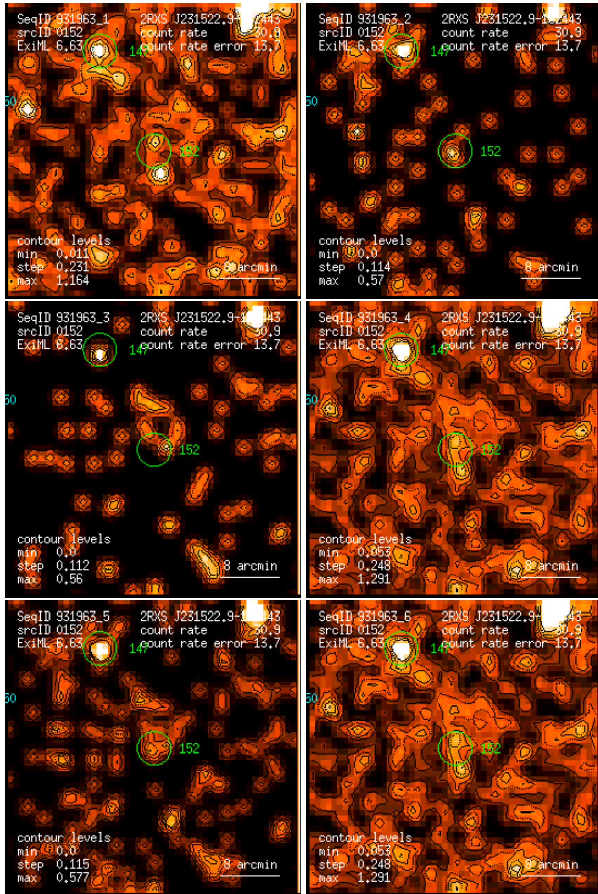
Figure 152: RASS 931963: detection 0152: band rate images, Gaussian filter: (1) PSPC channels 11 – 41, (2) 52 – 90, (3) 91 – 201, (4) 11 – 235, (5) 52 – 201, (6) 11 – 201. Broad band rates in counts/ks. Band rate contour levels in counts/ks/arcmin 2 .
