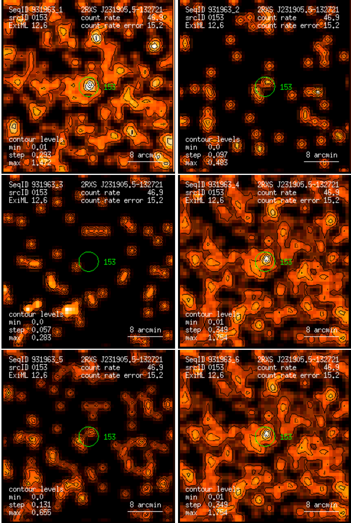
Figure 153: RASS 931963: detection 0153: band rate images, Gaussian filter: (1) PSPC channels 11 – 41, (2) 52 – 90, (3) 91 – 201, (4) 11 – 235, (5) 52 – 201, (6) 11 – 201. Broad band rates in counts/ks. Band rate contour levels in counts/ks/arcmin 2 .
