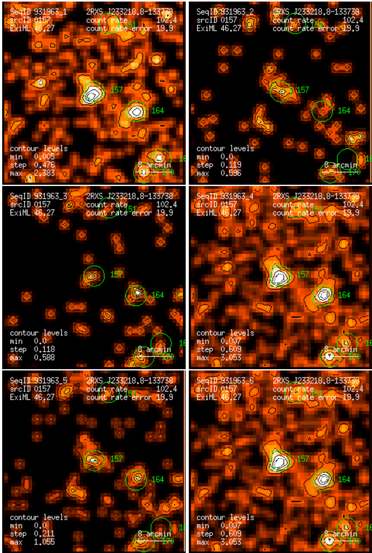
Figure 157: RASS 931963: detection 0157: band rate images, Gaussian filter: (1) PSPC channels 11 – 41, (2) 52 – 90, (3) 91 – 201, (4) 11 – 235, (5) 52 – 201, (6) 11 – 201. Broad band rates in counts/ks. Band rate contour levels in counts/ks/arcmin 2 .
