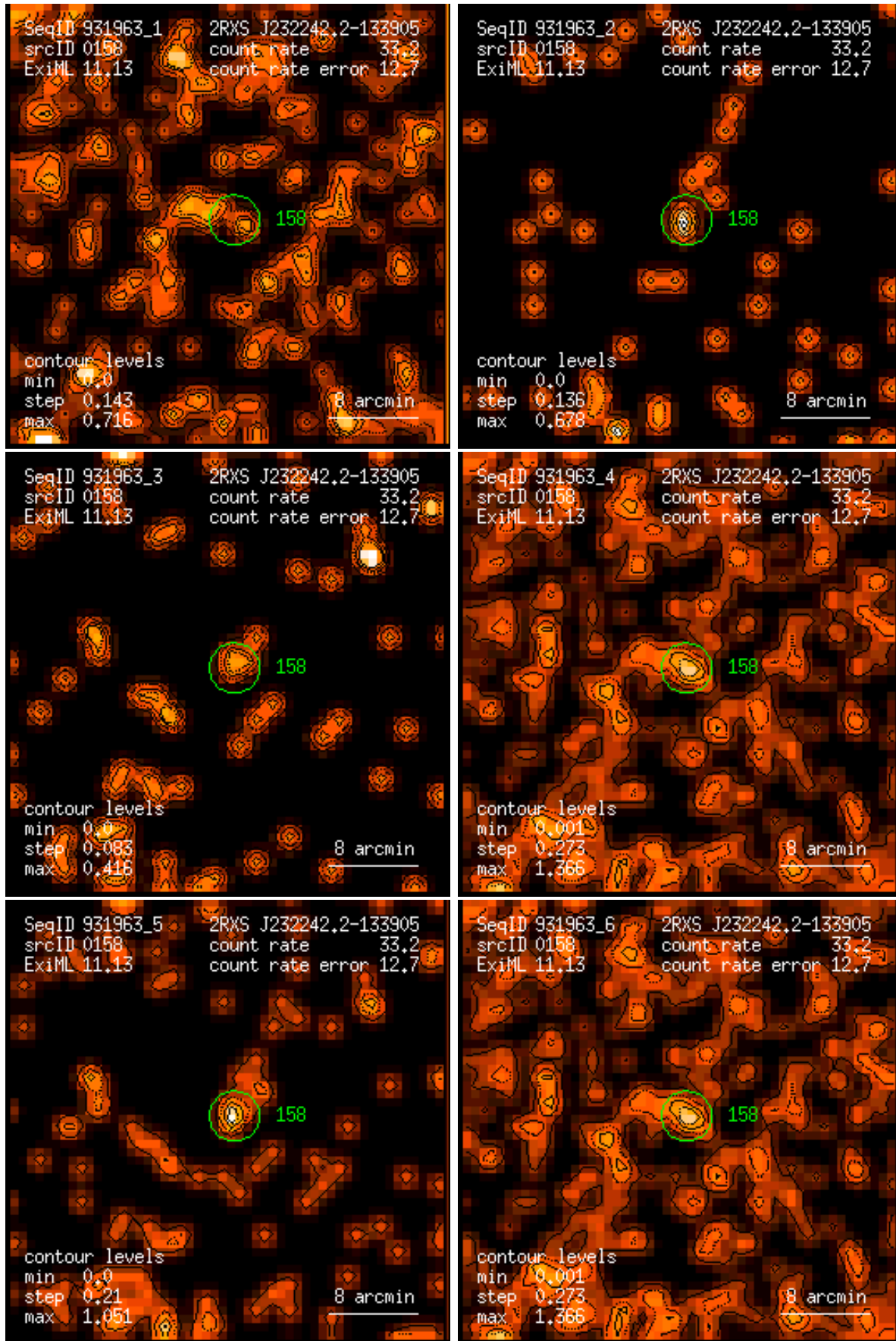
Figure 158: RASS 931963: detection 0158: band rate images, Gaussian filter: (1) PSPC channels 11 – 41, (2) 52 – 90, (3) 91 – 201, (4) 11 – 235, (5) 52 – 201, (6) 11 – 201. Broad band rates in counts/ks. Band rate contour levels in counts/ks/arcmin 2 .
