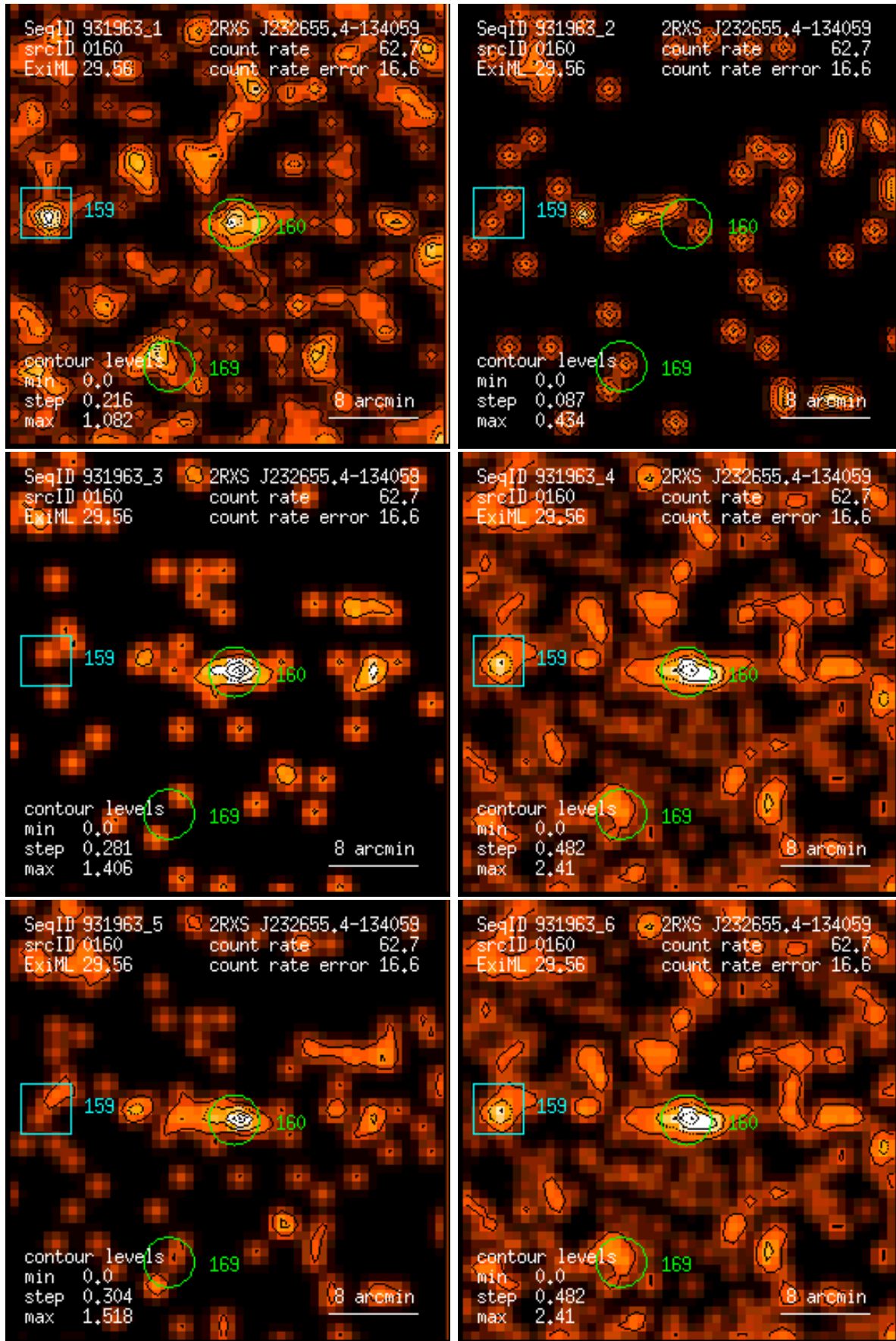
Figure 160: RASS 931963: detection 0160: band rate images, Gaussian filter: (1) PSPC channels 11 – 41, (2) 52 – 90, (3) 91 – 201, (4) 11 – 235, (5) 52 – 201, (6) 11 – 201. Broad band rates in counts/ks. Band rate contour levels in counts/ks/arcmin 2 .
