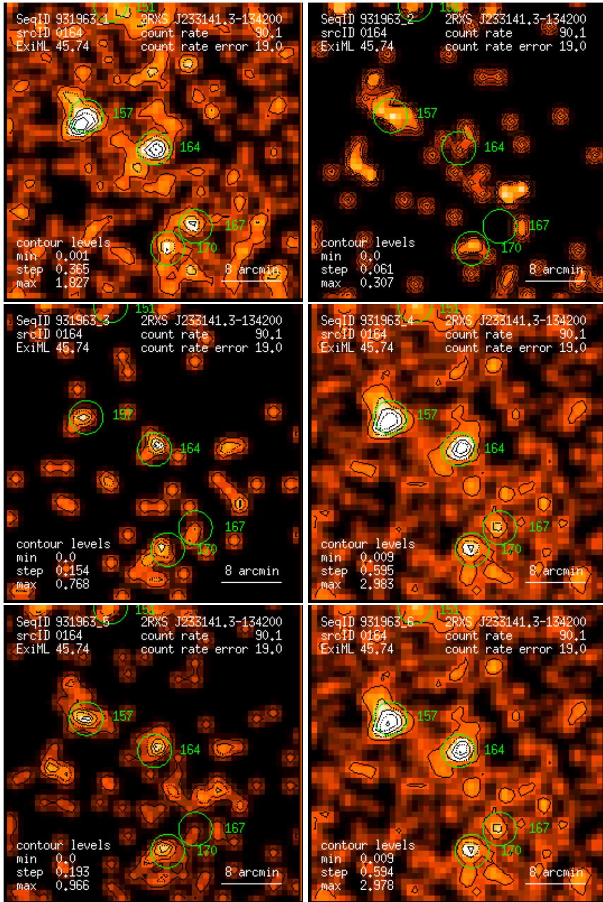
Figure 164: RASS 931963: detection 0164: band rate images, Gaussian filter: (1) PSPC channels 11 – 41, (2) 52 – 90, (3) 91 – 201, (4) 11 – 235, (5) 52 – 201, (6) 11 – 201. Broad band rates in counts/ks. Band rate contour levels in counts/ks/arcmin 2 .
