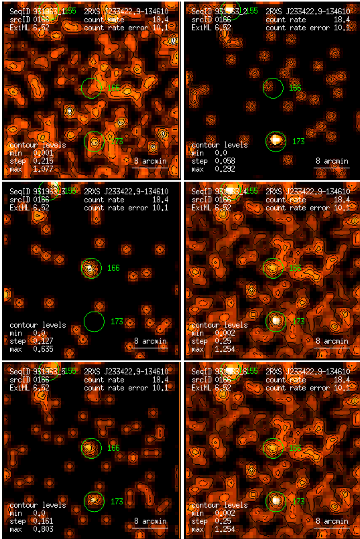
Figure 166: RASS 931963: detection 0166: band rate images, Gaussian filter: (1) PSPC channels 11 – 41, (2) 52 – 90, (3) 91 – 201, (4) 11 – 235, (5) 52 – 201, (6) 11 – 201. Broad band rates in counts/ks. Band rate contour levels in counts/ks/arcmin 2 .
