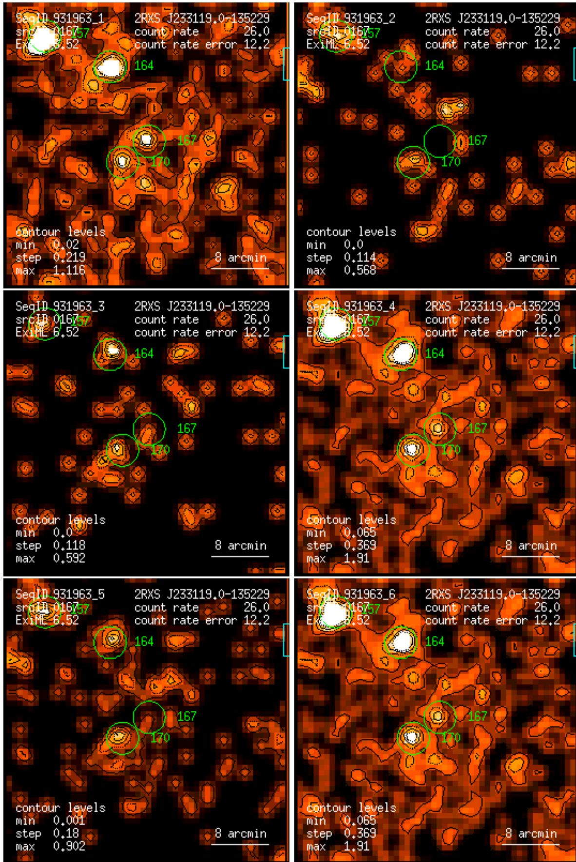
Figure 167: RASS 931963: detection 0167: band rate images, Gaussian filter: (1) PSPC channels 11 – 41, (2) 52 – 90, (3) 91 – 201, (4) 11 – 235, (5) 52 – 201, (6) 11 – 201. Broad band rates in counts/ks. Band rate contour levels in counts/ks/arcmin 2 .
