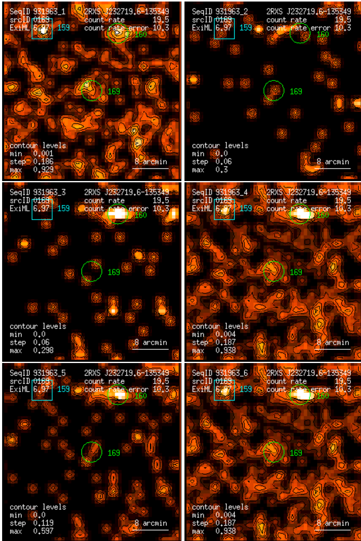
Figure 169: RASS 931963: detection 0169: band rate images, Gaussian filter: (1) PSPC channels 11 – 41, (2) 52 – 90, (3) 91 – 201, (4) 11 – 235, (5) 52 – 201, (6) 11 – 201. Broad band rates in counts/ks. Band rate contour levels in counts/ks/arcmin 2 .
