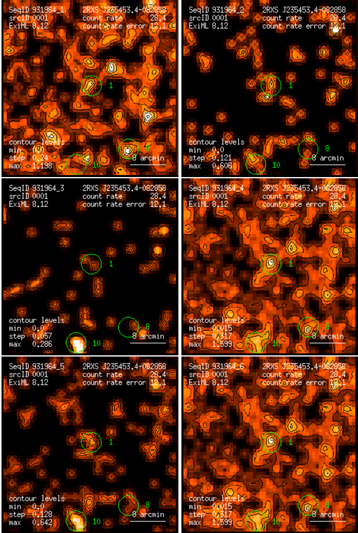
Figure 1: RASS 931964: detection 0001: band rate images, Gaussian filter: (1) PSPC channels 11 – 41, (2) 52 – 90, (3) 91 – 201, (4) 11 – 235, (5) 52 – 201, (6) 11 – 201. Broad band rates in counts/ks. Band rate contour levels in counts/ks/arcmin 2 .
