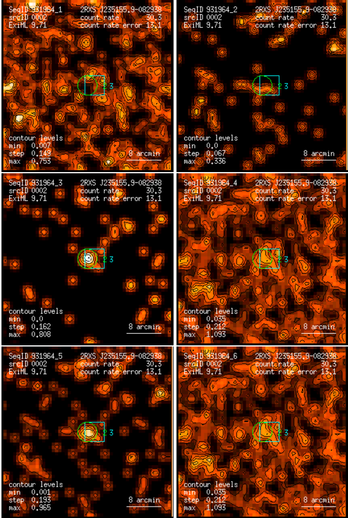
Figure 2: RASS 931964: detection 0002: band rate images, Gaussian filter: (1) PSPC channels 11 – 41, (2) 52 – 90, (3) 91 – 201, (4) 11 – 235, (5) 52 – 201, (6) 11 – 201. Broad band rates in counts/ks. Band rate contour levels in counts/ks/arcmin 2 .
