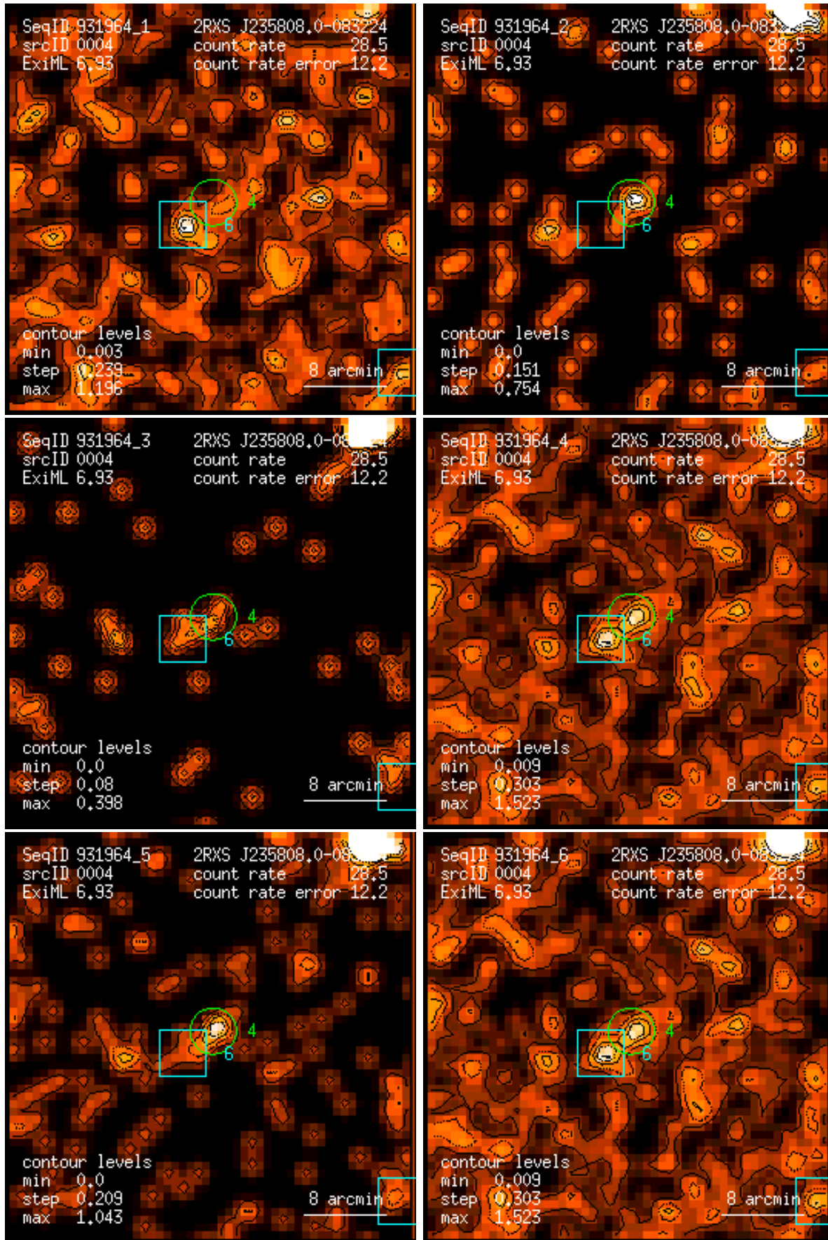
Figure 4: RASS 931964: detection 0004: band rate images, Gaussian filter: (1) PSPC channels 11 – 41, (2) 52 – 90, (3) 91 – 201, (4) 11 – 235, (5) 52 – 201, (6) 11 – 201. Broad band rates in counts/ks. Band rate contour levels in counts/ks/arcmin 2 .
