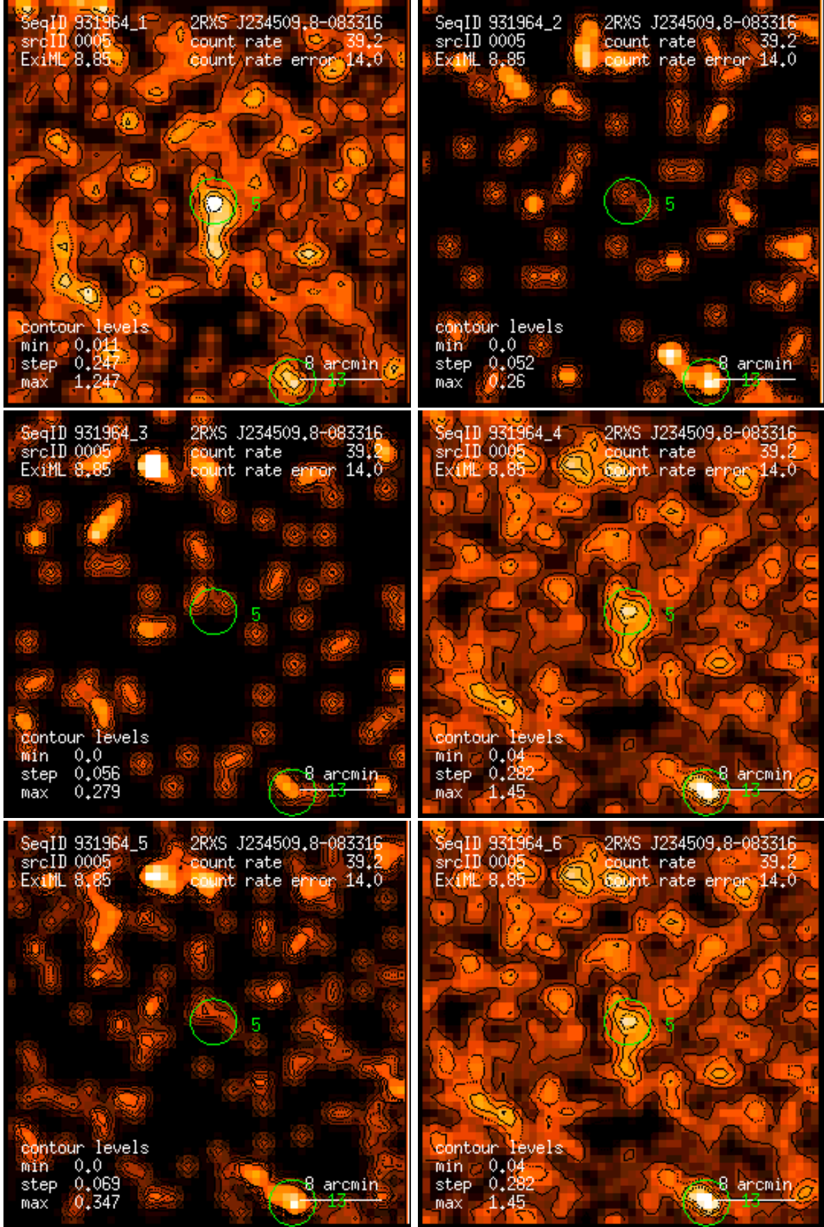
Figure 5: RASS 931964: detection 0005: band rate images, Gaussian filter: (1) PSPC channels 11 – 41, (2) 52 – 90, (3) 91 – 201, (4) 11 – 235, (5) 52 – 201, (6) 11 – 201. Broad band rates in counts/ks. Band rate contour levels in counts/ks/arcmin 2 .
